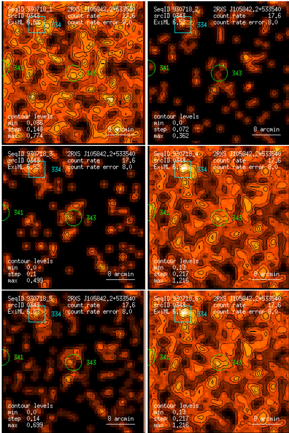
Figure 343: RASS 930718: detection 0343: band rate images, Gaussian filter: (1) PSPC channels 11 – 41, (2) 52 – 90, (3) 91 – 201, (4) 11 – 235, (5) 52 – 201, (6) 11 – 201. Broad band rates in counts/ks. Band rate contour levels in counts/ks/arcmin 2 .
