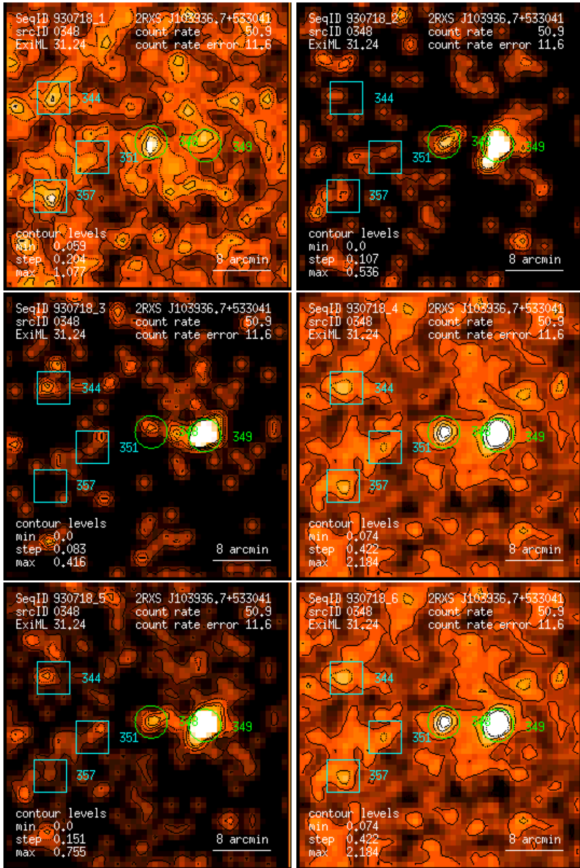
Figure 348: RASS 930718: detection 0348: band rate images, Gaussian filter: (1) PSPC channels 11 – 41, (2) 52 – 90, (3) 91 – 201, (4) 11 – 235, (5) 52 – 201, (6) 11 – 201. Broad band rates in counts/ks. Band rate contour levels in counts/ks/arcmin 2 .
