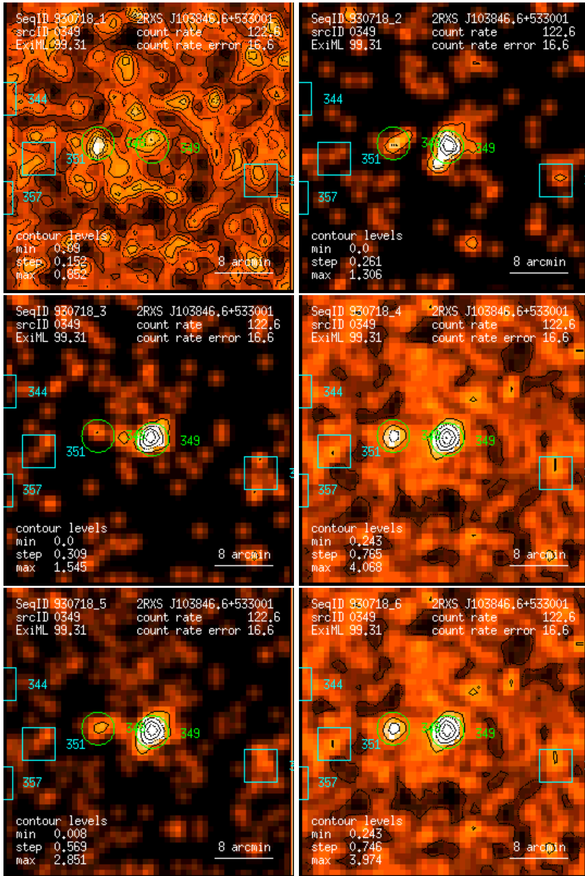
Figure 349: RASS 930718: detection 0349: band rate images, Gaussian filter: (1) PSPC channels 11 – 41, (2) 52 – 90, (3) 91 – 201, (4) 11 – 235, (5) 52 – 201, (6) 11 – 201. Broad band rates in counts/ks. Band rate contour levels in counts/ks/arcmin 2 .
