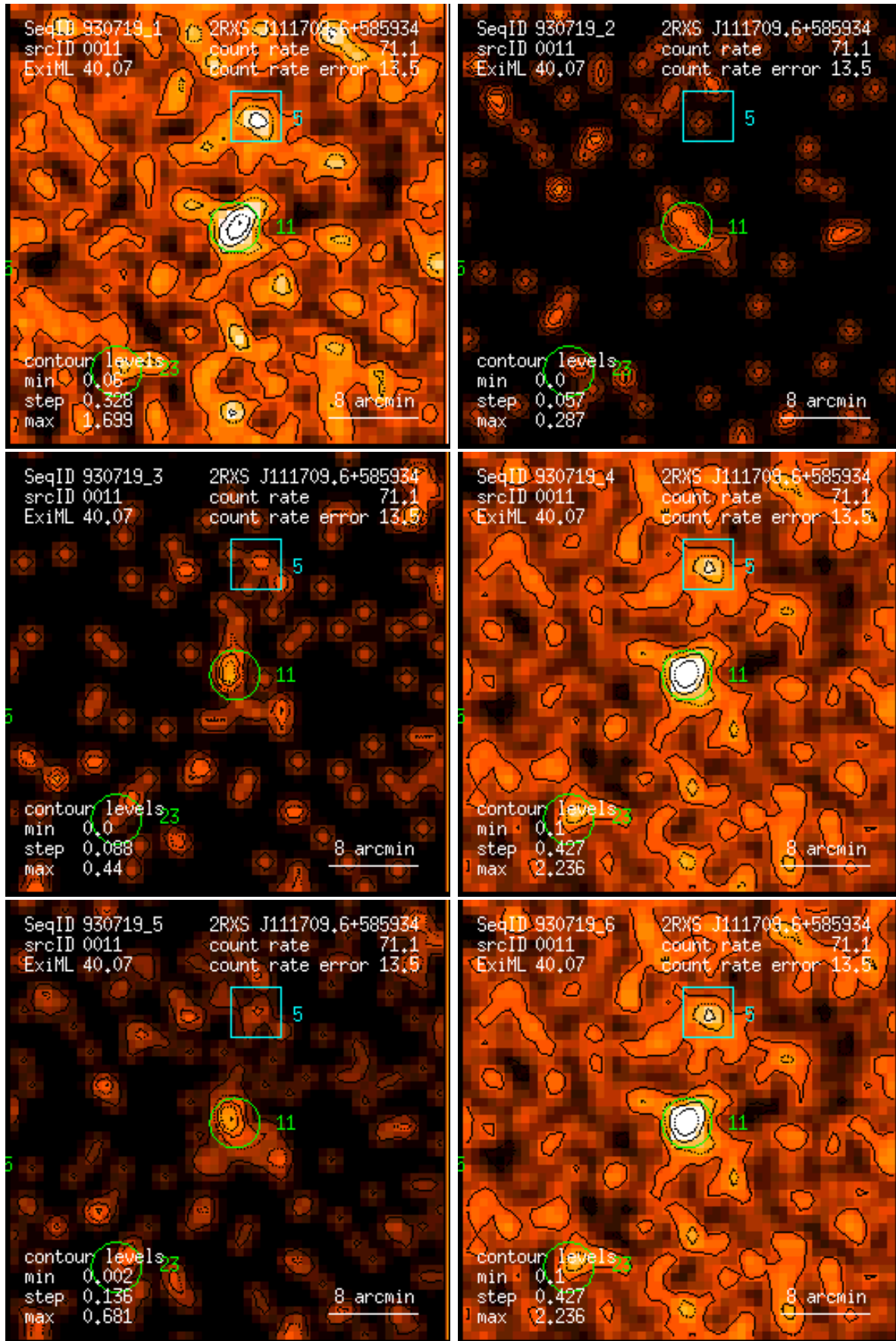
Figure 11: RASS 930719: detection 0011: band rate images, Gaussian filter: (1) PSPC channels 11 – 41, (2) 52 – 90, (3) 91 – 201, (4) 11 – 235, (5) 52 – 201, (6) 11 – 201. Broad band rates in counts/ks. Band rate contour levels in counts/ks/arcmin 2 .
