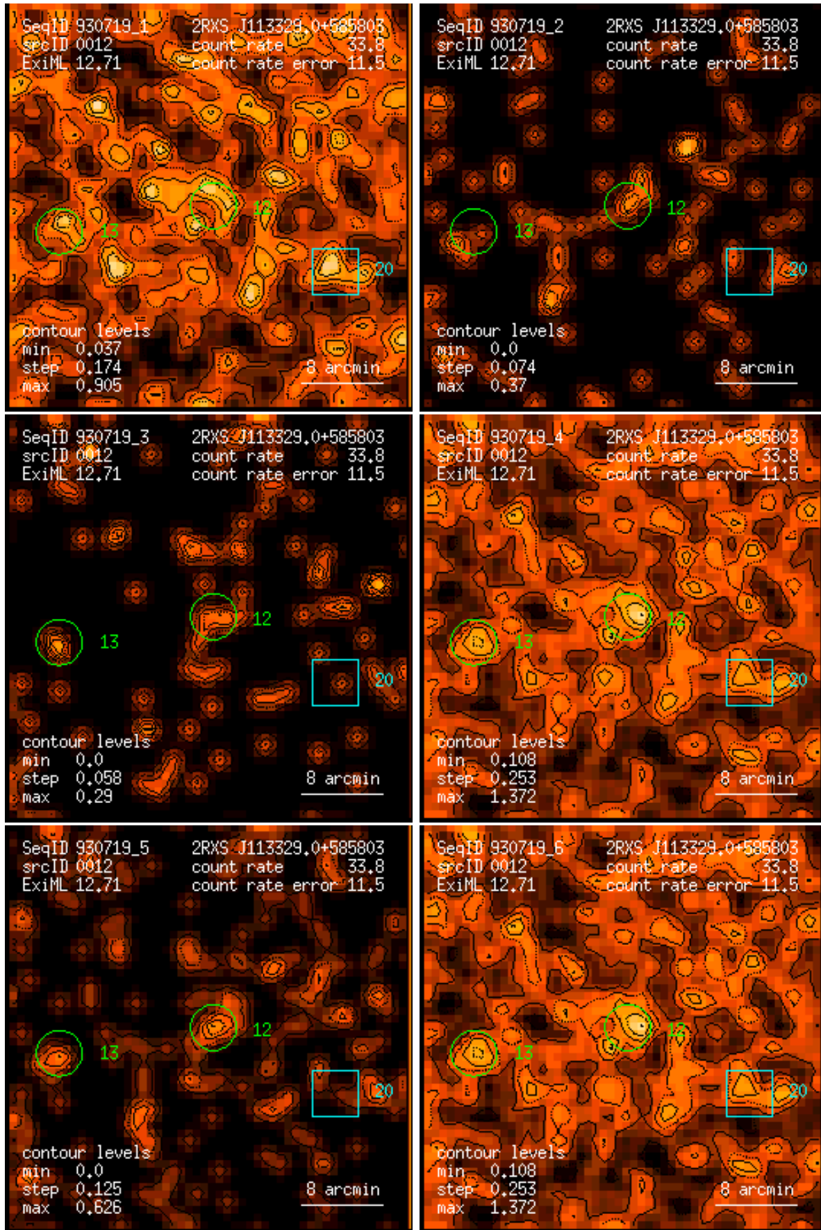
Figure 12: RASS 930719: detection 0012: band rate images, Gaussian filter: (1) PSPC channels 11 – 41, (2) 52 – 90, (3) 91 – 201, (4) 11 – 235, (5) 52 – 201, (6) 11 – 201. Broad band rates in counts/ks. Band rate contour levels in counts/ks/arcmin 2 .
