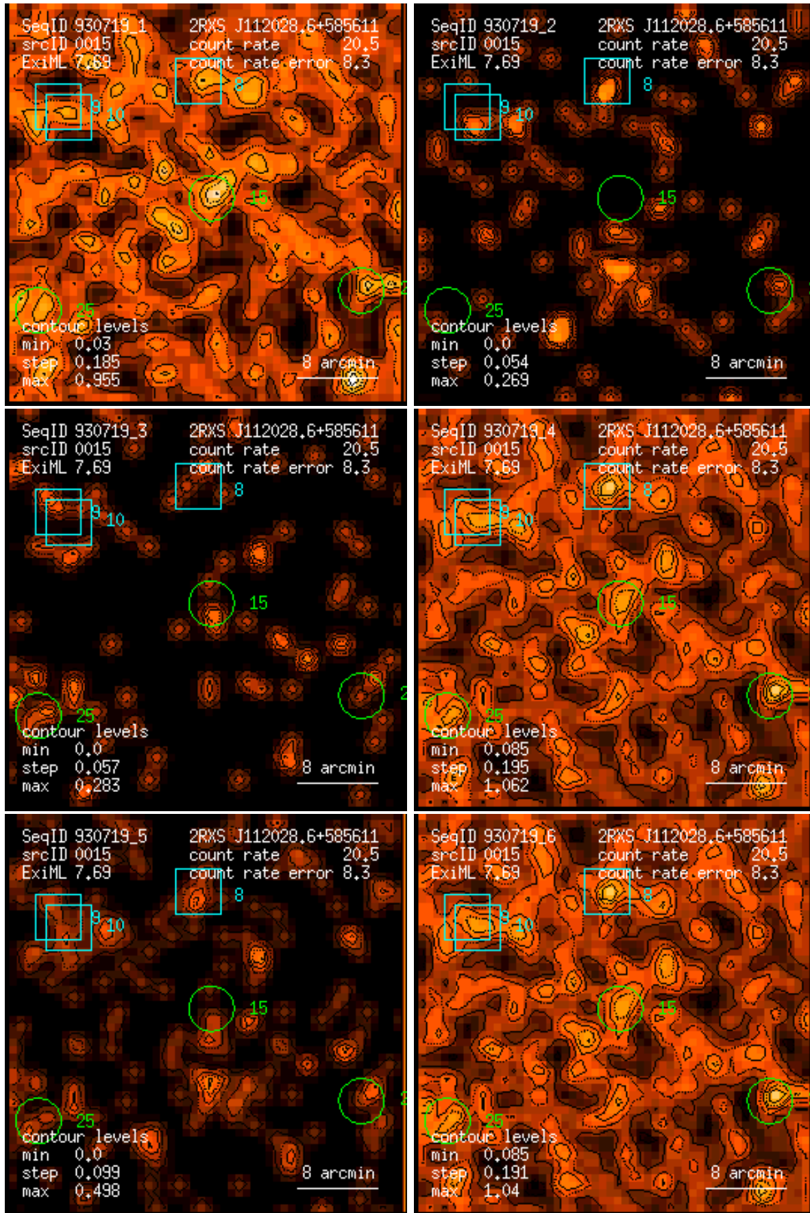
Figure 15: RASS 930719: detection 0015: band rate images, Gaussian filter: (1) PSPC channels 11 – 41, (2) 52 – 90, (3) 91 – 201, (4) 11 – 235, (5) 52 – 201, (6) 11 – 201. Broad band rates in counts/ks. Band rate contour levels in counts/ks/arcmin 2 .
