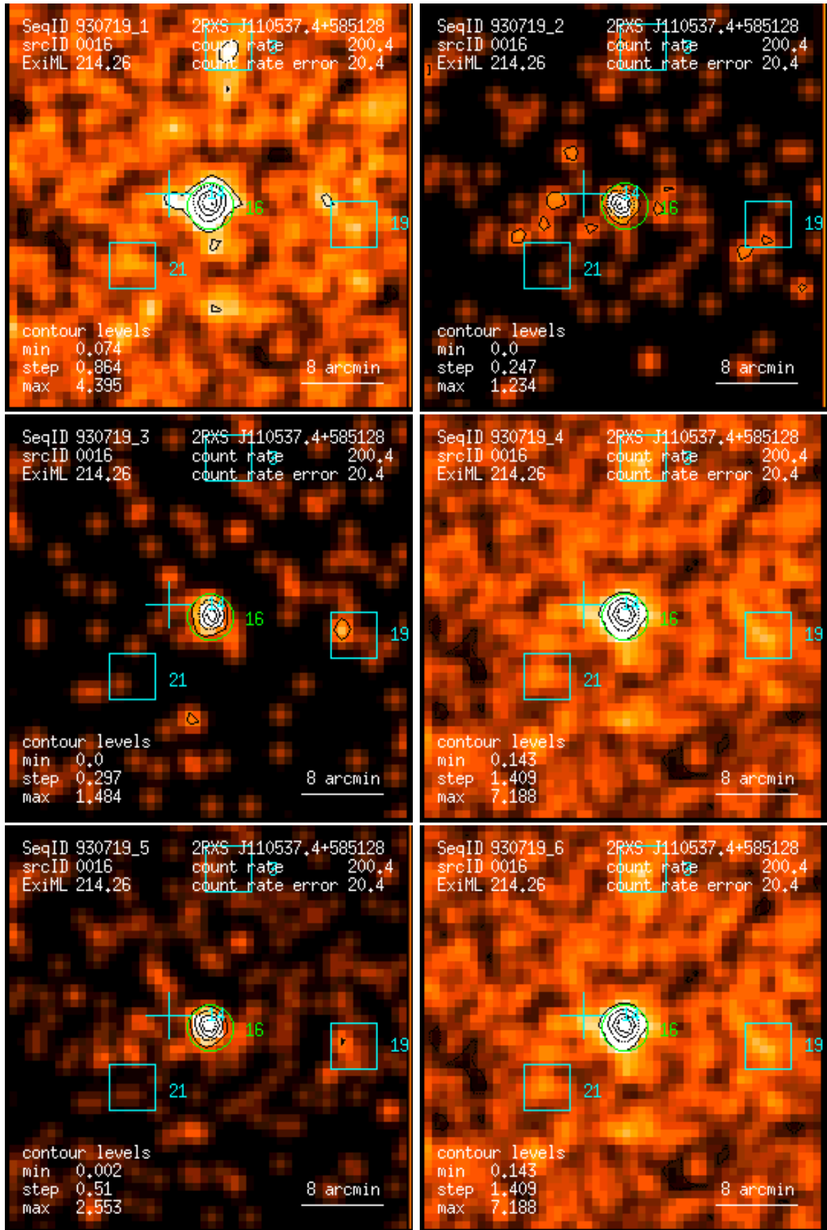
Figure 16: RASS 930719: detection 0016: band rate images, Gaussian filter: (1) PSPC channels 11 – 41, (2) 52 – 90, (3) 91 – 201, (4) 11 – 235, (5) 52 – 201, (6) 11 – 201. Broad band rates in counts/ks. Band rate contour levels in counts/ks/arcmin 2 .
