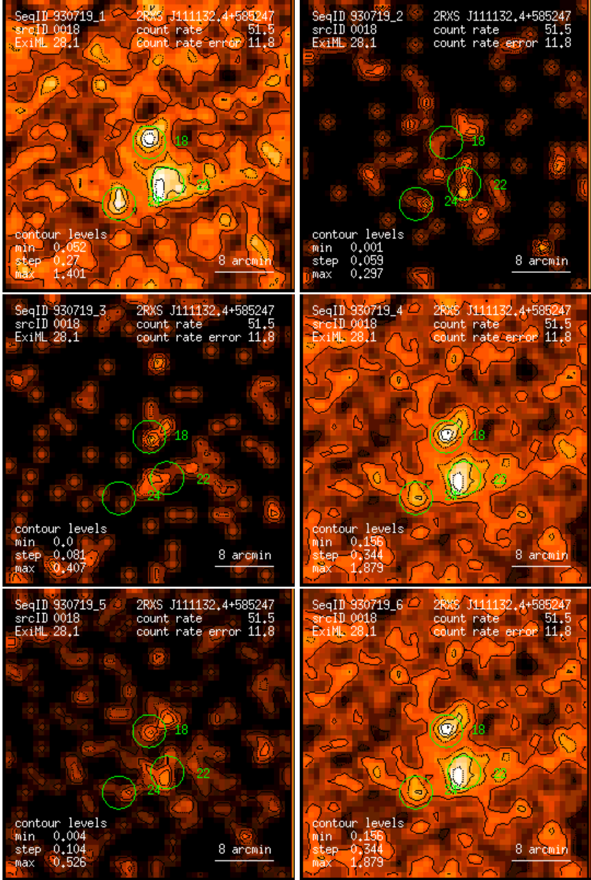
Figure 18: RASS 930719: detection 0018: band rate images, Gaussian filter: (1) PSPC channels 11 – 41, (2) 52 – 90, (3) 91 – 201, (4) 11 – 235, (5) 52 – 201, (6) 11 – 201. Broad band rates in counts/ks. Band rate contour levels in counts/ks/arcmin 2 .
