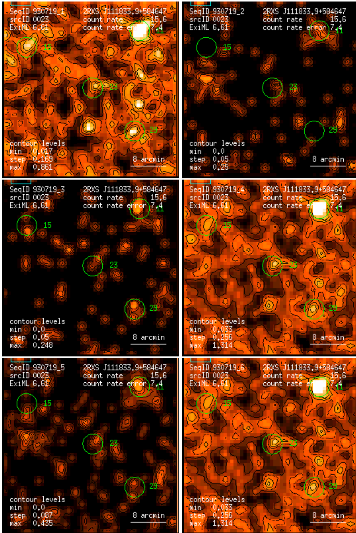
Figure 23: RASS 930719: detection 0023: band rate images, Gaussian filter: (1) PSPC channels 11 – 41, (2) 52 – 90, (3) 91 – 201, (4) 11 – 235, (5) 52 – 201, (6) 11 – 201. Broad band rates in counts/ks. Band rate contour levels in counts/ks/arcmin 2 .
