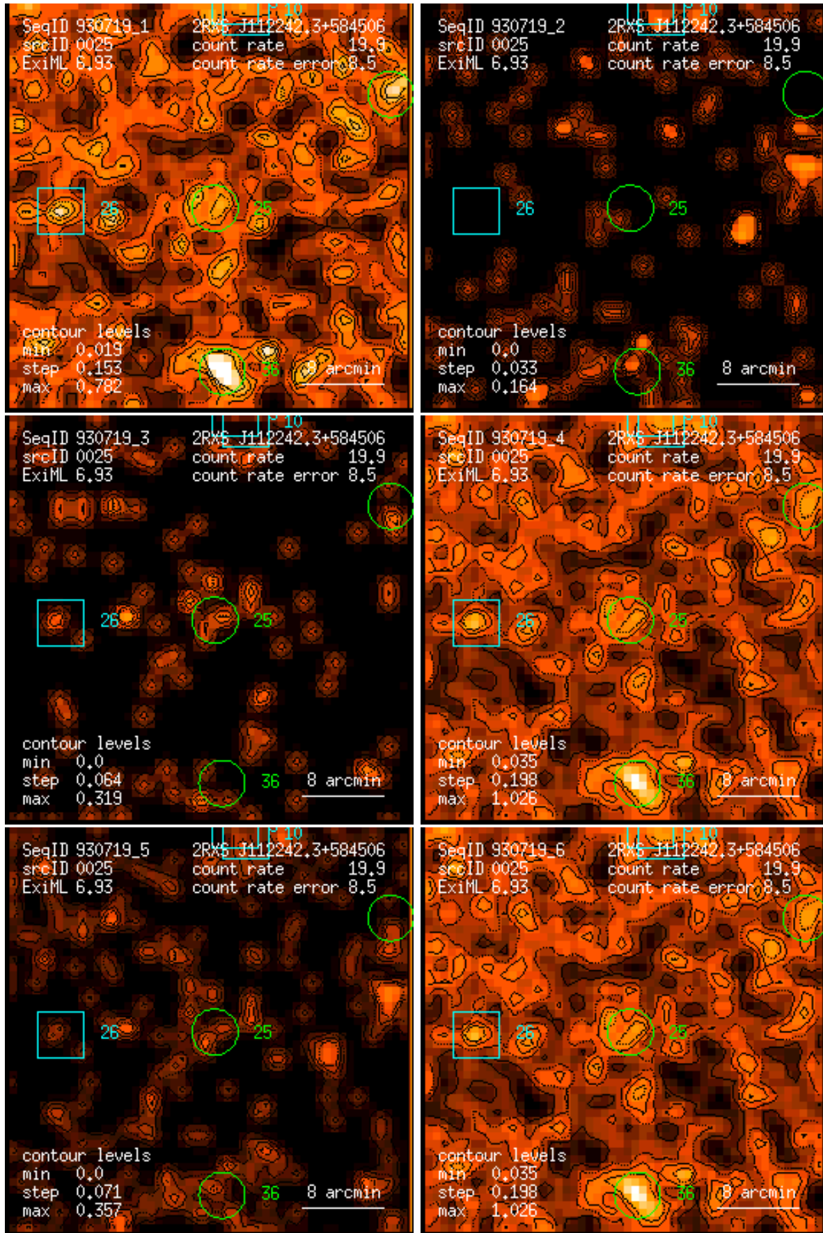
Figure 25: RASS 930719: detection 0025: band rate images, Gaussian filter: (1) PSPC channels 11 – 41, (2) 52 – 90, (3) 91 – 201, (4) 11 – 235, (5) 52 – 201, (6) 11 – 201. Broad band rates in counts/ks. Band rate contour levels in counts/ks/arcmin 2 .
