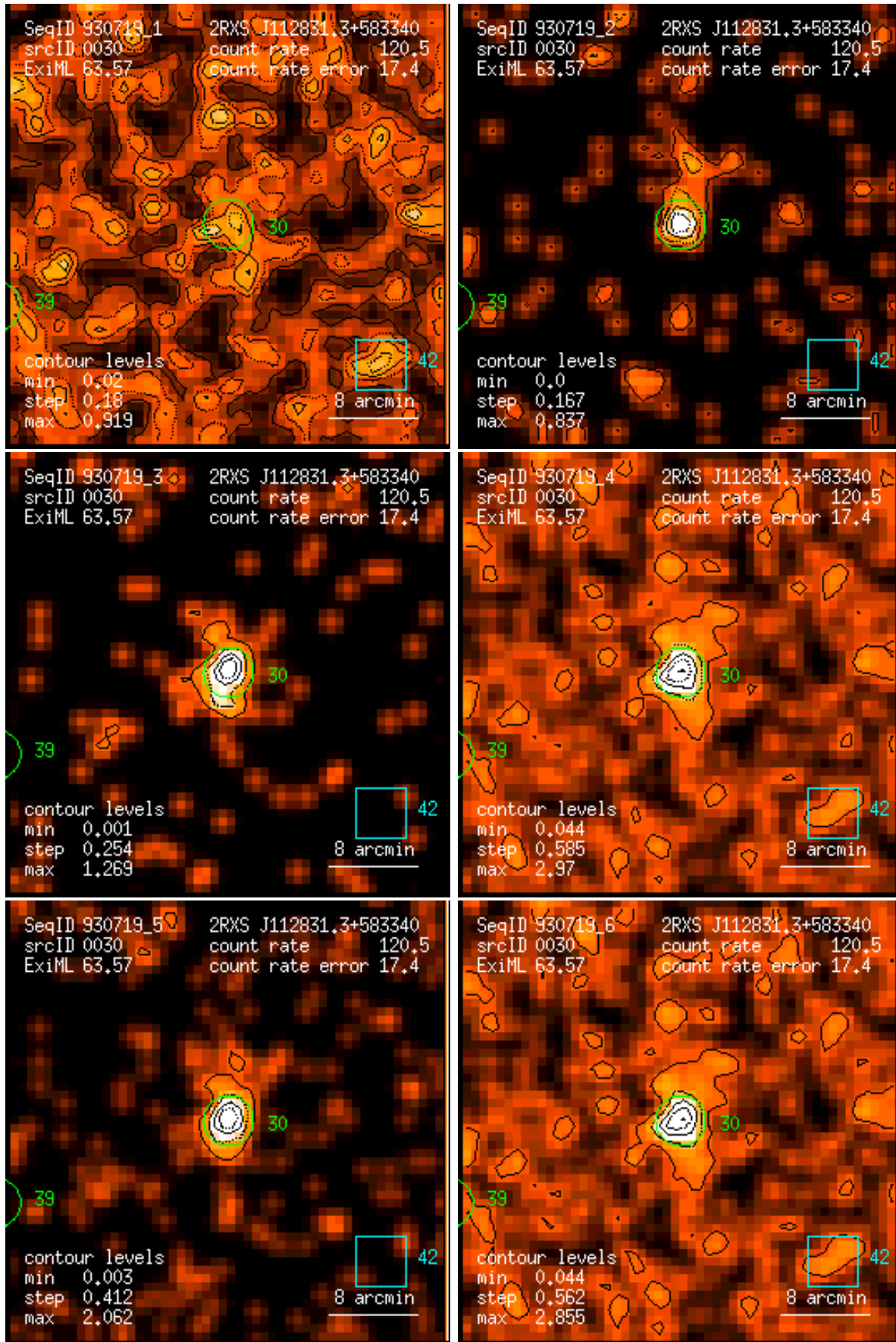
Figure 30: RASS 930719: detection 0030: band rate images, Gaussian filter: (1) PSPC channels 11 – 41, (2) 52 – 90, (3) 91 – 201, (4) 11 – 235, (5) 52 – 201, (6) 11 – 201. Broad band rates in counts/ks. Band rate contour levels in counts/ks/arcmin 2 .
