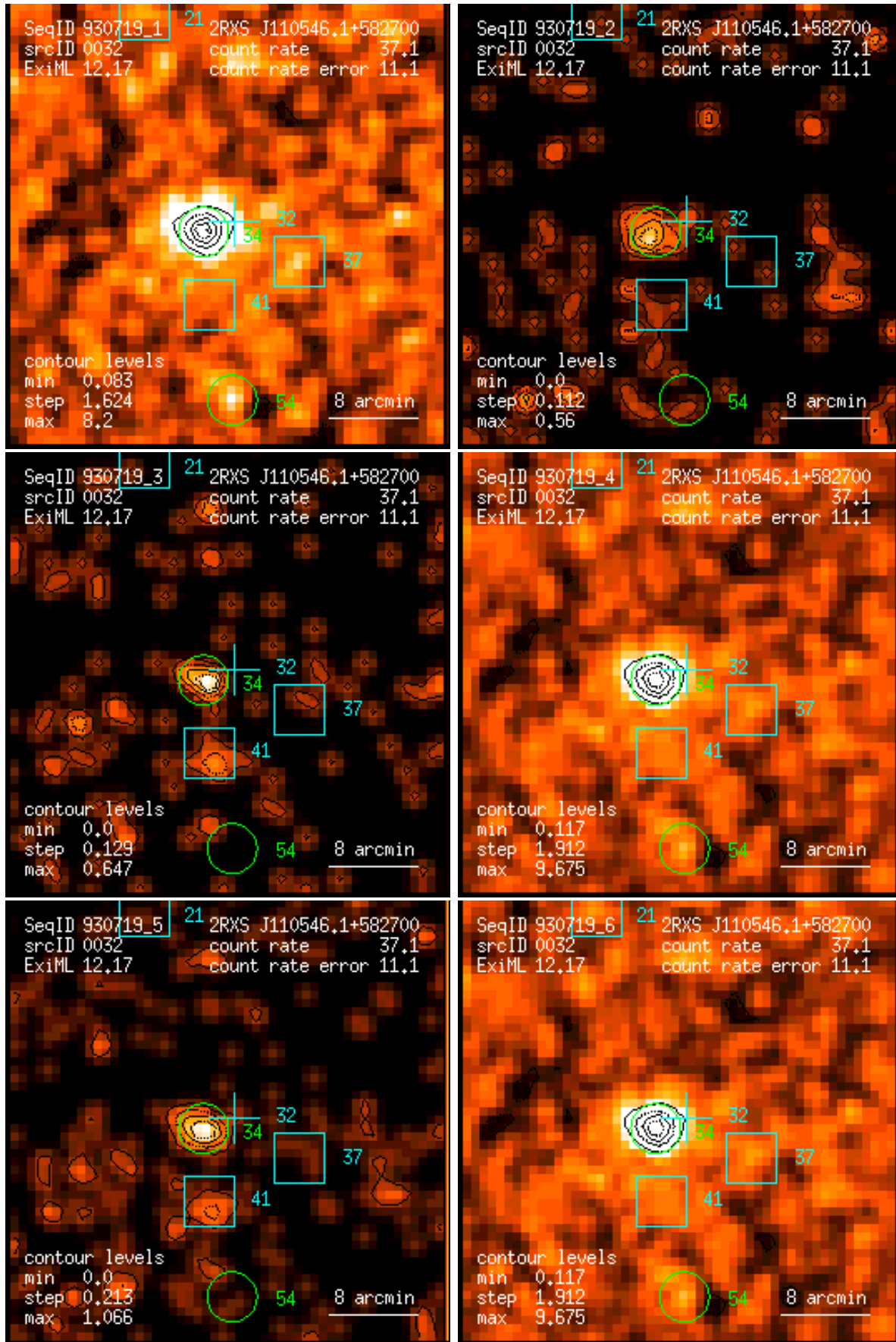
Figure 32: RASS 930719: detection 0032: band rate images, Gaussian filter: (1) PSPC channels 11 – 41, (2) 52 – 90, (3) 91 – 201, (4) 11 – 235, (5) 52 – 201, (6) 11 – 201. Broad band rates in counts/ks. Band rate contour levels in counts/ks/arcmin 2 .
