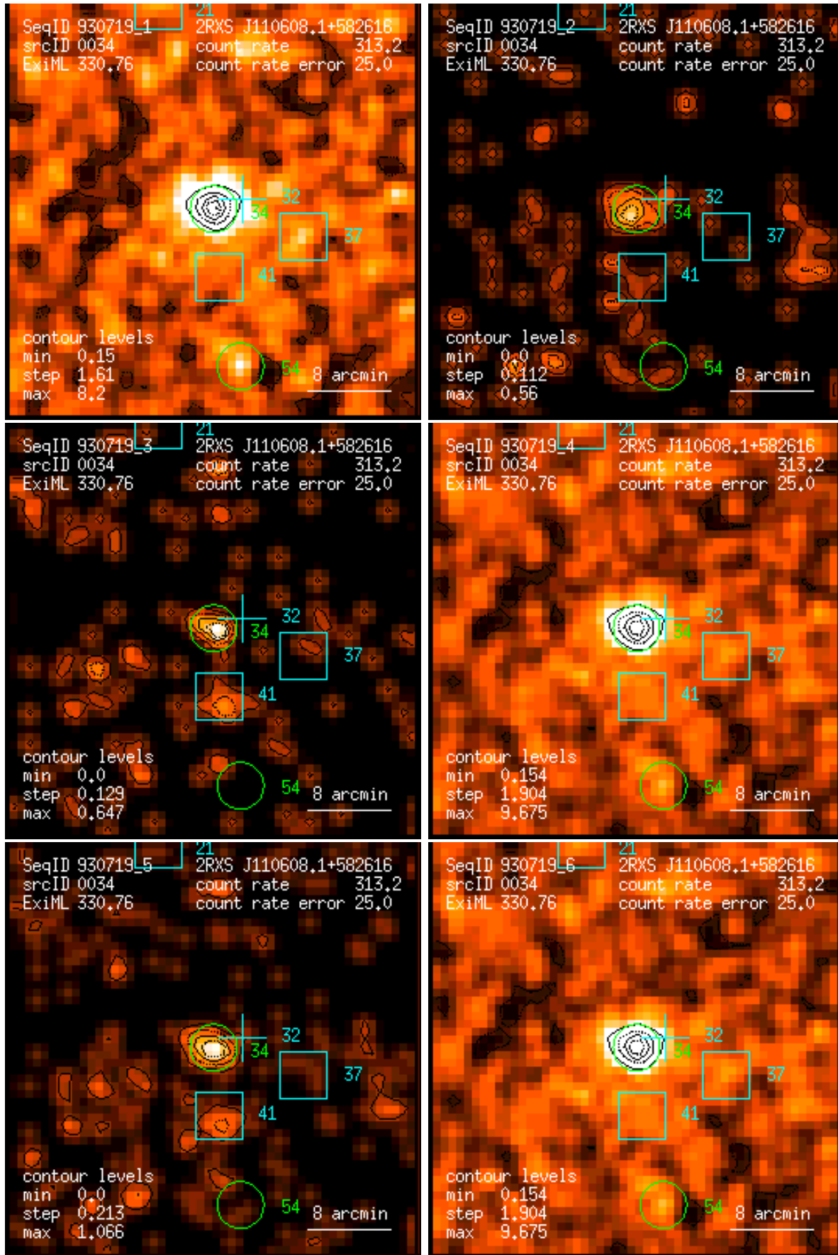
Figure 34: RASS 930719: detection 0034: band rate images, Gaussian filter: (1) PSPC channels 11 – 41, (2) 52 – 90, (3) 91 – 201, (4) 11 – 235, (5) 52 – 201, (6) 11 – 201. Broad band rates in counts/ks. Band rate contour levels in counts/ks/arcmin 2 .
