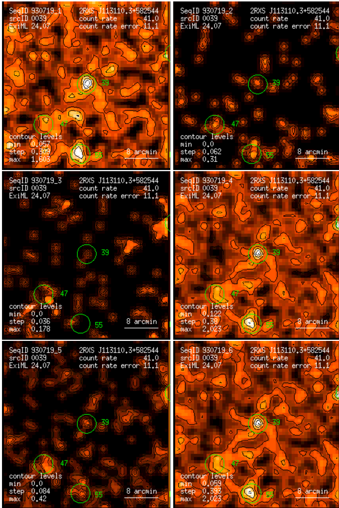
Figure 39: RASS 930719: detection 0039: band rate images, Gaussian filter: (1) PSPC channels 11 – 41, (2) 52 – 90, (3) 91 – 201, (4) 11 – 235, (5) 52 – 201, (6) 11 – 201. Broad band rates in counts/ks. Band rate contour levels in counts/ks/arcmin 2 .
