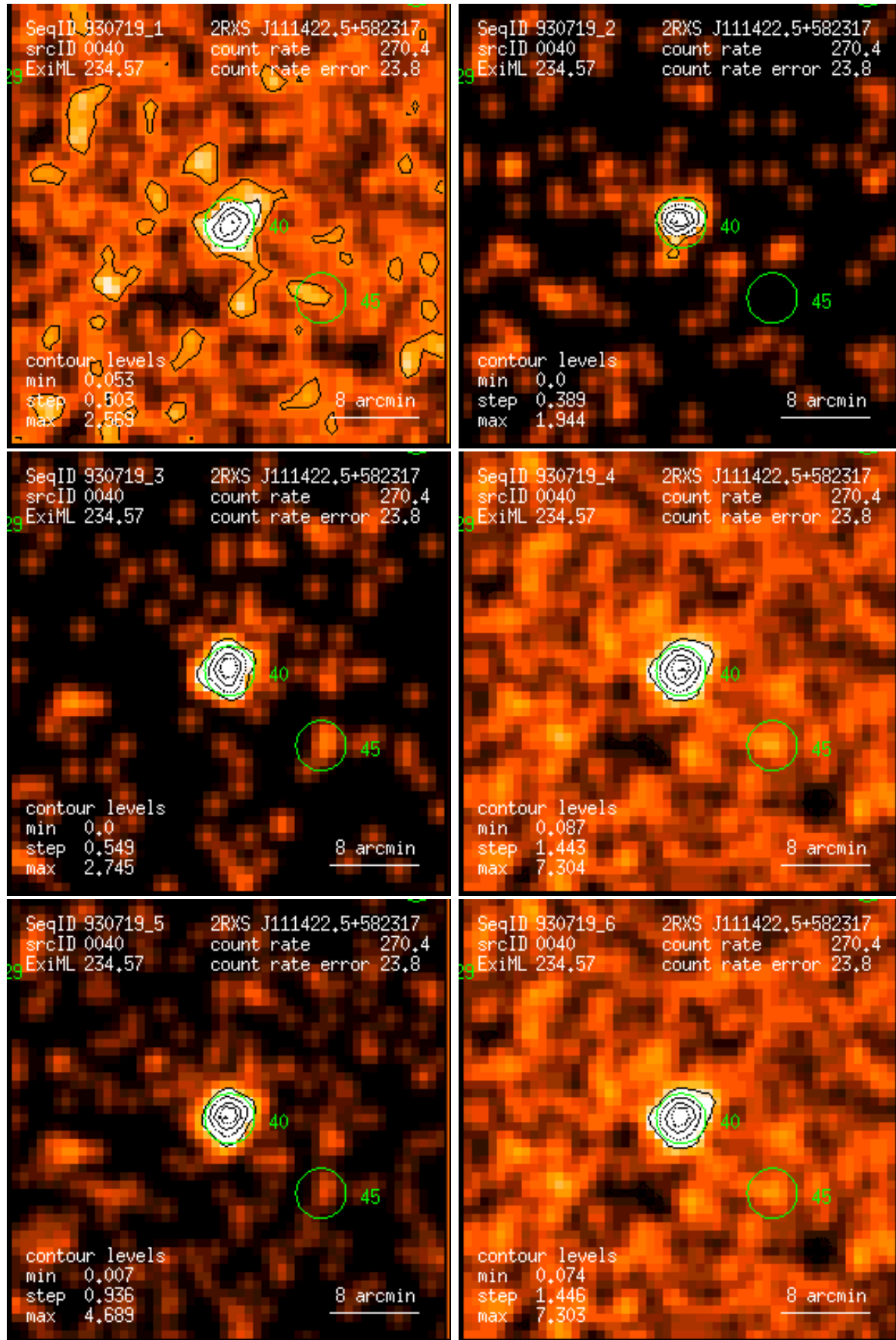
Figure 40: RASS 930719: detection 0040: band rate images, Gaussian filter: (1) PSPC channels 11 – 41, (2) 52 – 90, (3) 91 – 201, (4) 11 – 235, (5) 52 – 201, (6) 11 – 201. Broad band rates in counts/ks. Band rate contour levels in counts/ks/arcmin 2 .
