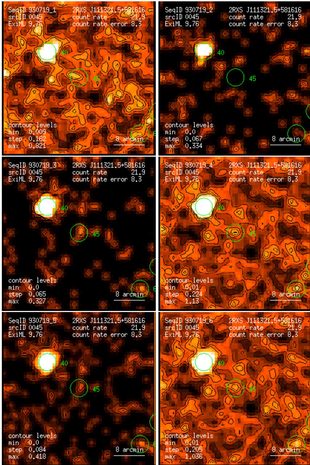
Figure 45: RASS 930719: detection 0045: band rate images, Gaussian filter: (1) PSPC channels 11 – 41, (2) 52 – 90, (3) 91 – 201, (4) 11 – 235, (5) 52 – 201, (6) 11 – 201. Broad band rates in counts/ks. Band rate contour levels in counts/ks/arcmin 2 .
