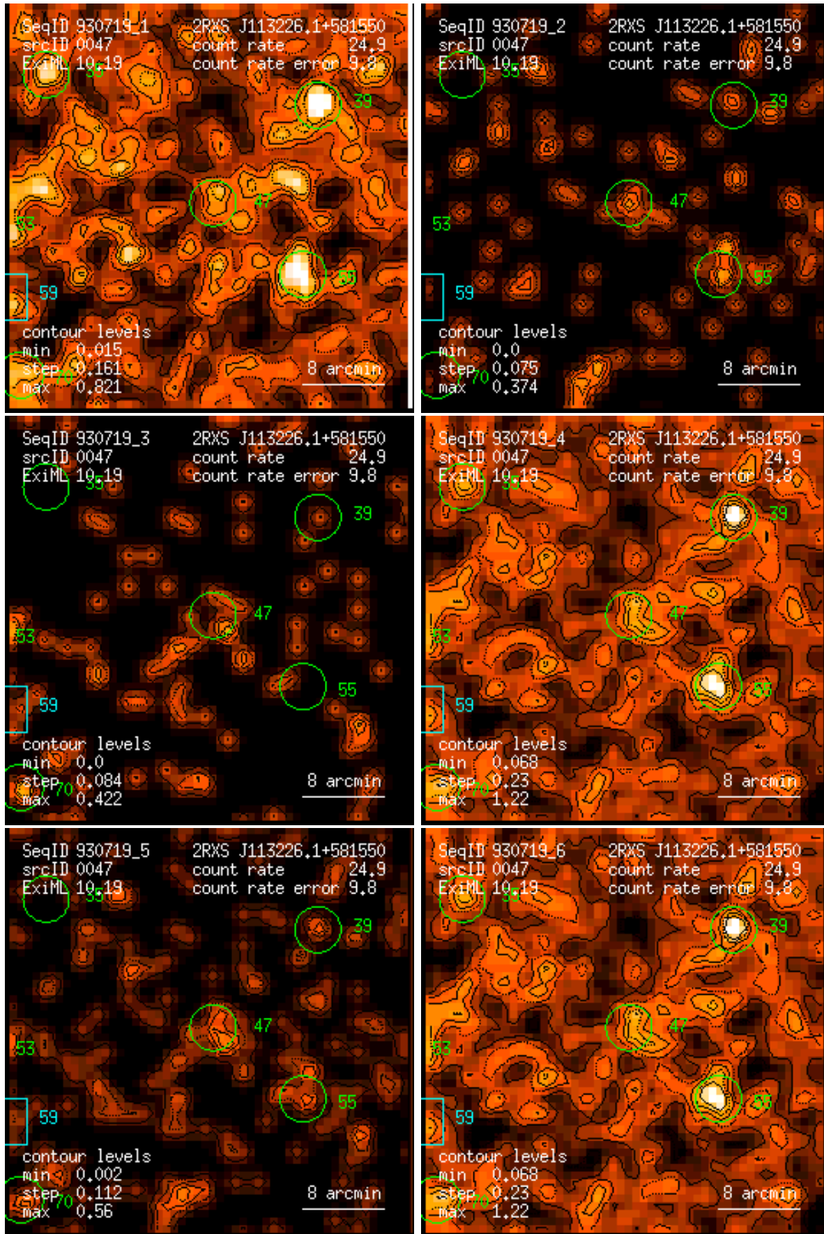
Figure 47: RASS 930719: detection 0047: band rate images, Gaussian filter: (1) PSPC channels 11 – 41, (2) 52 – 90, (3) 91 – 201, (4) 11 – 235, (5) 52 – 201, (6) 11 – 201. Broad band rates in counts/ks. Band rate contour levels in counts/ks/arcmin 2 .
