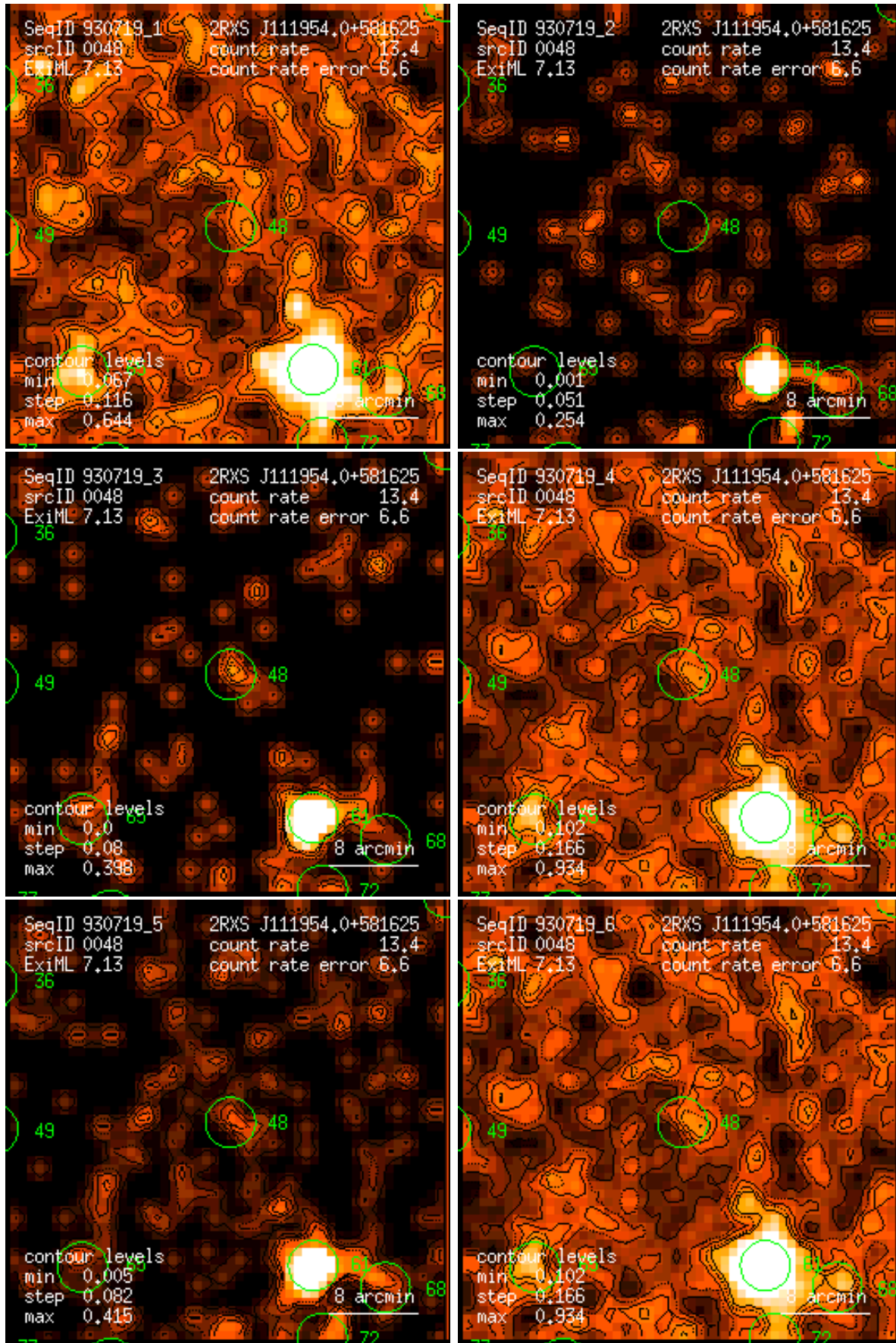
Figure 48: RASS 930719: detection 0048: band rate images, Gaussian filter: (1) PSPC channels 11 – 41, (2) 52 – 90, (3) 91 – 201, (4) 11 – 235, (5) 52 – 201, (6) 11 – 201. Broad band rates in counts/ks. Band rate contour levels in counts/ks/arcmin 2 .
