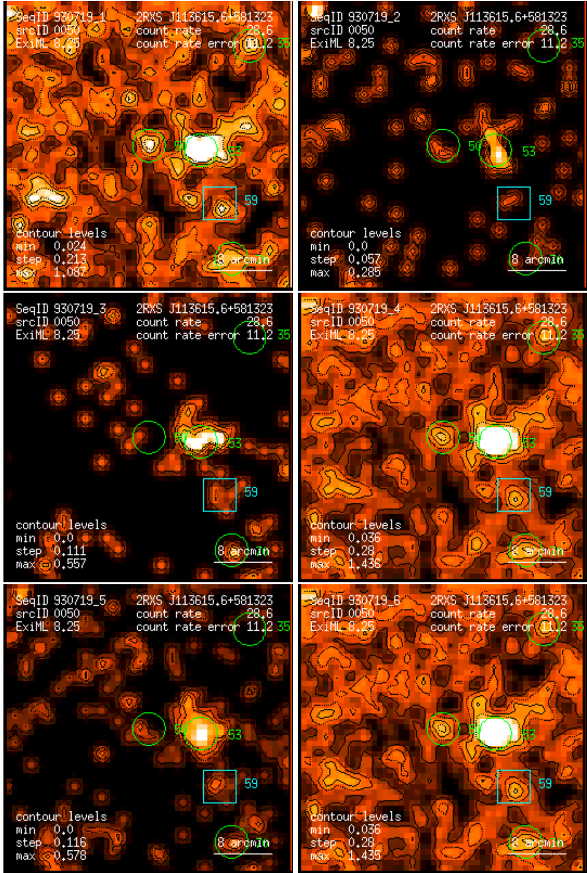
Figure 50: RASS 930719: detection 0050: band rate images, Gaussian filter: (1) PSPC channels 11 – 41, (2) 52 – 90, (3) 91 – 201, (4) 11 – 235, (5) 52 – 201, (6) 11 – 201. Broad band rates in counts/ks. Band rate contour levels in counts/ks/arcmin 2 .
