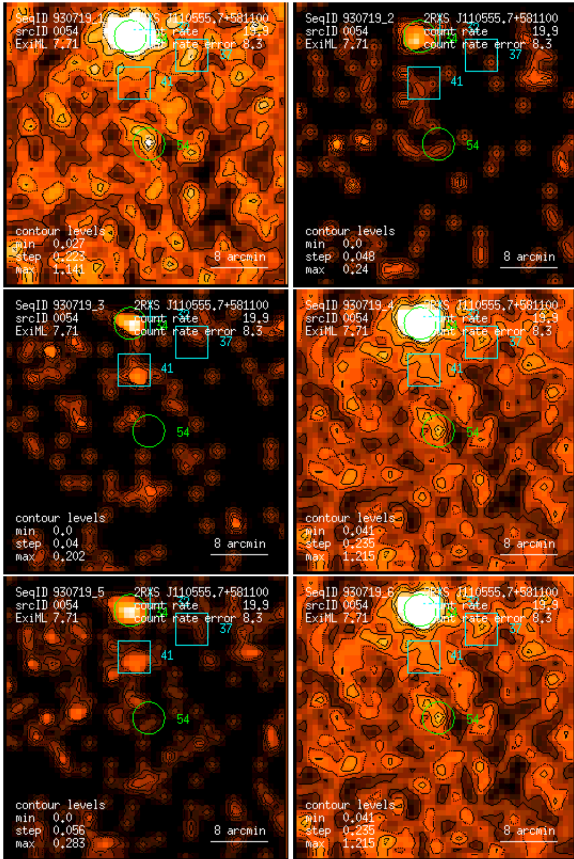
Figure 54: RASS 930719: detection 0054: band rate images, Gaussian filter: (1) PSPC channels 11 – 41, (2) 52 – 90, (3) 91 – 201, (4) 11 – 235, (5) 52 – 201, (6) 11 – 201. Broad band rates in counts/ks. Band rate contour levels in counts/ks/arcmin 2 .
