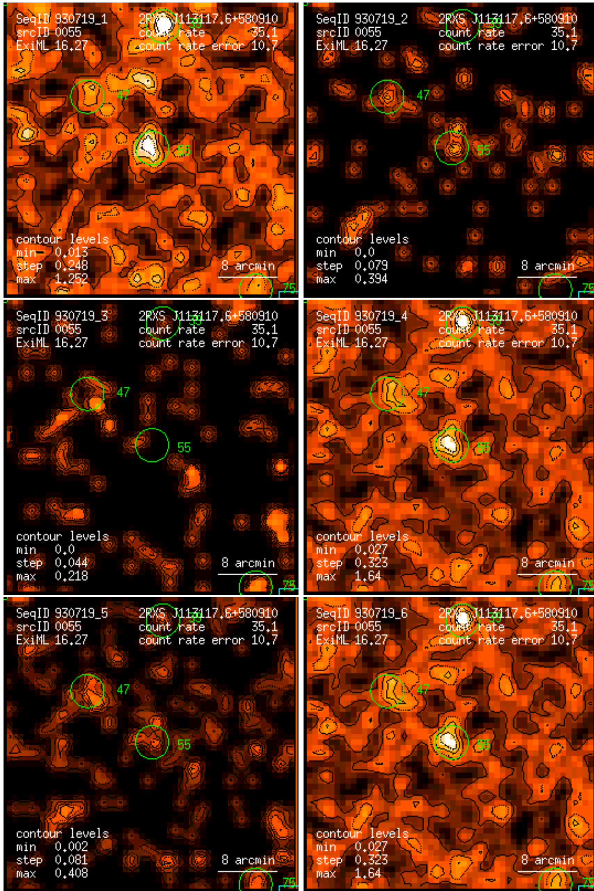
Figure 55: RASS 930719: detection 0055: band rate images, Gaussian filter: (1) PSPC channels 11 – 41, (2) 52 – 90, (3) 91 – 201, (4) 11 – 235, (5) 52 – 201, (6) 11 – 201. Broad band rates in counts/ks. Band rate contour levels in counts/ks/arcmin 2 .
