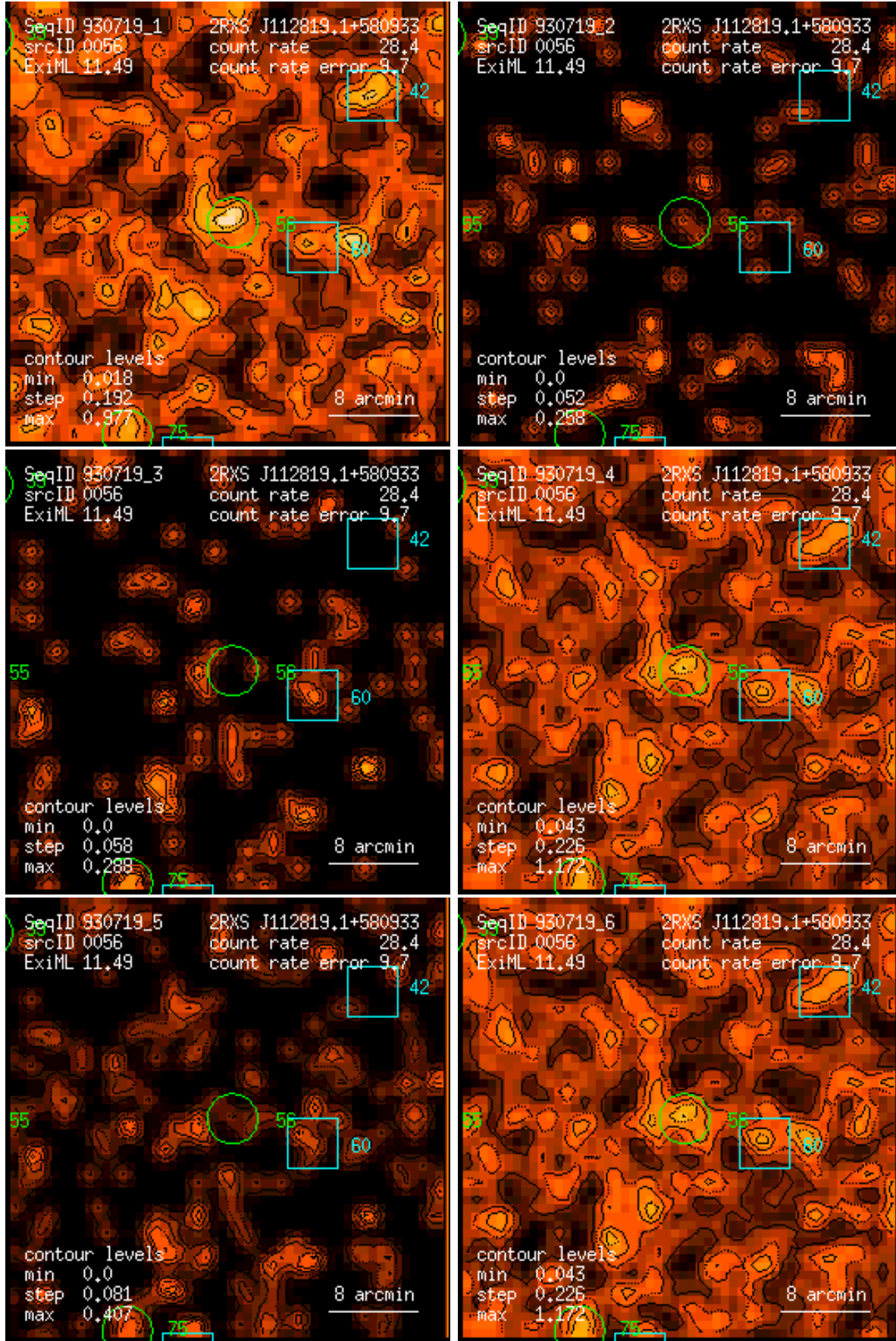
Figure 56: RASS 930719: detection 0056: band rate images, Gaussian filter: (1) PSPC channels 11 – 41, (2) 52 – 90, (3) 91 – 201, (4) 11 – 235, (5) 52 – 201, (6) 11 – 201. Broad band rates in counts/ks. Band rate contour levels in counts/ks/arcmin 2 .
