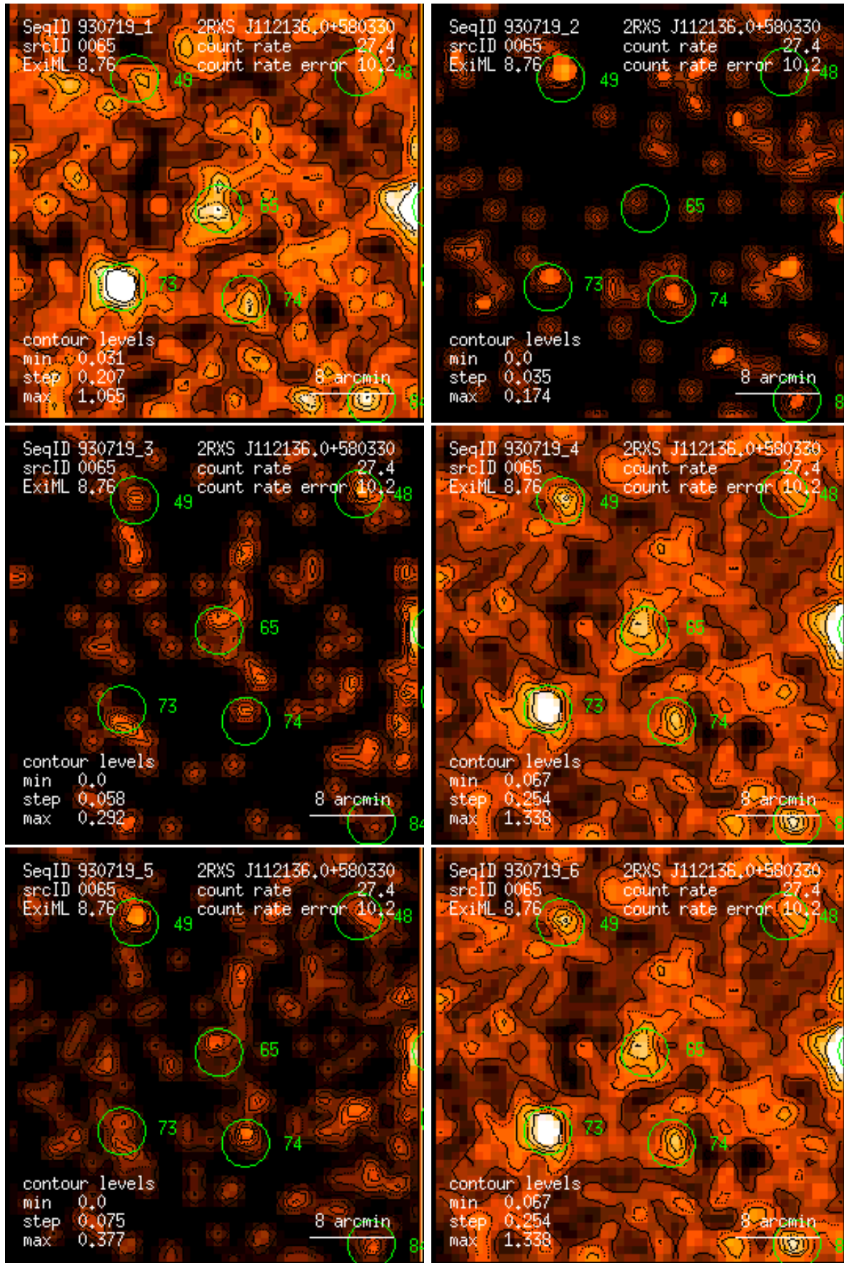
Figure 65: RASS 930719: detection 0065: band rate images, Gaussian filter: (1) PSPC channels 11 – 41, (2) 52 – 90, (3) 91 – 201, (4) 11 – 235, (5) 52 – 201, (6) 11 – 201. Broad band rates in counts/ks. Band rate contour levels in counts/ks/arcmin 2 .
