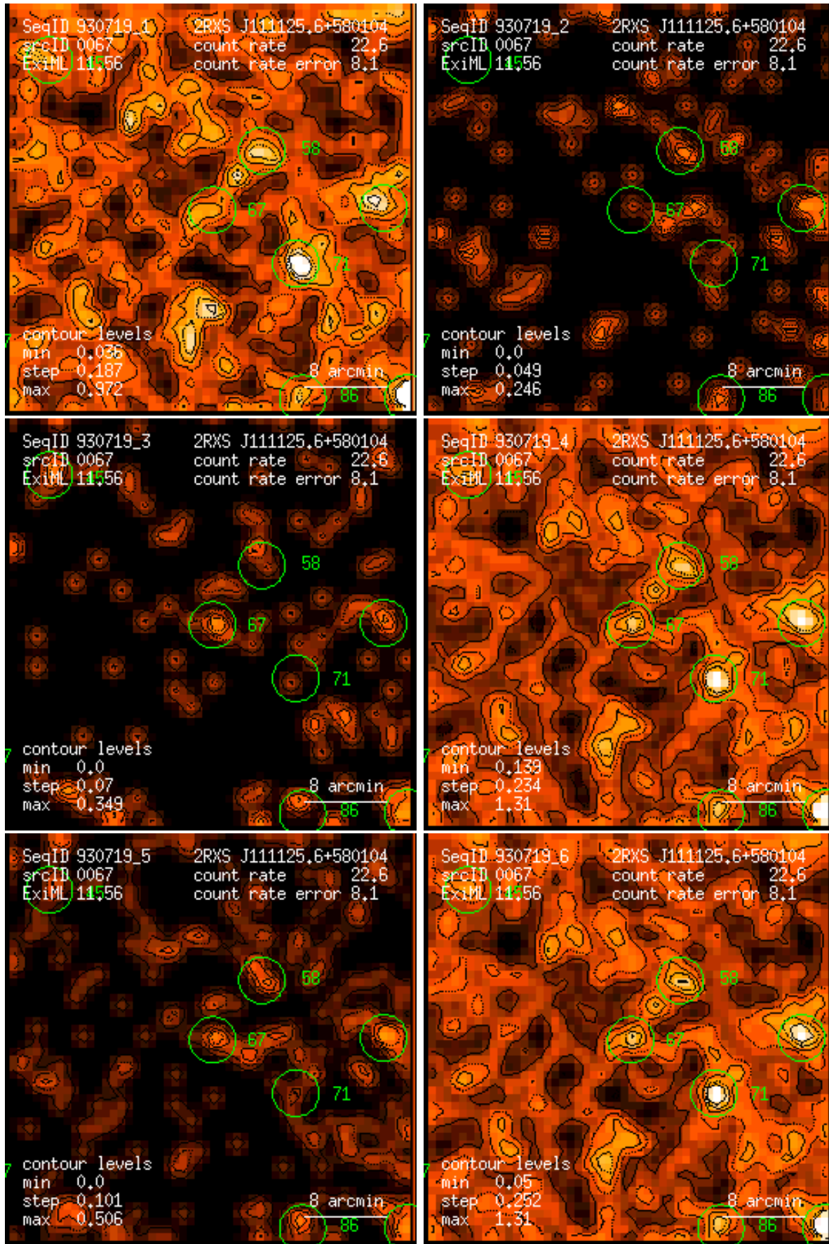
Figure 67: RASS 930719: detection 0067: band rate images, Gaussian filter: (1) PSPC channels 11 – 41, (2) 52 – 90, (3) 91 – 201, (4) 11 – 235, (5) 52 – 201, (6) 11 – 201. Broad band rates in counts/ks. Band rate contour levels in counts/ks/arcmin 2 .
