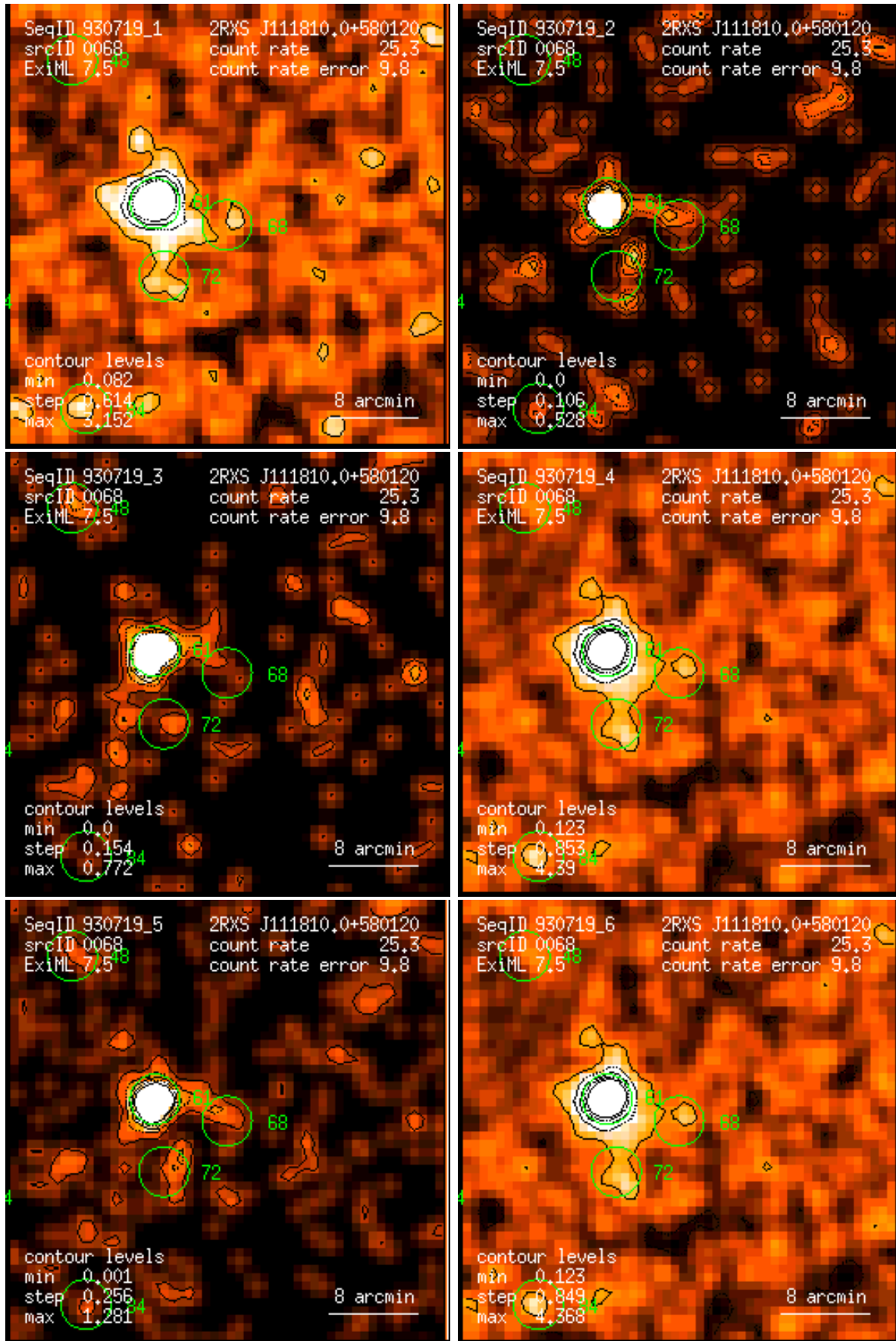
Figure 68: RASS 930719: detection 0068: band rate images, Gaussian filter: (1) PSPC channels 11 – 41, (2) 52 – 90, (3) 91 – 201, (4) 11 – 235, (5) 52 – 201, (6) 11 – 201. Broad band rates in counts/ks. Band rate contour levels in counts/ks/arcmin 2 .
