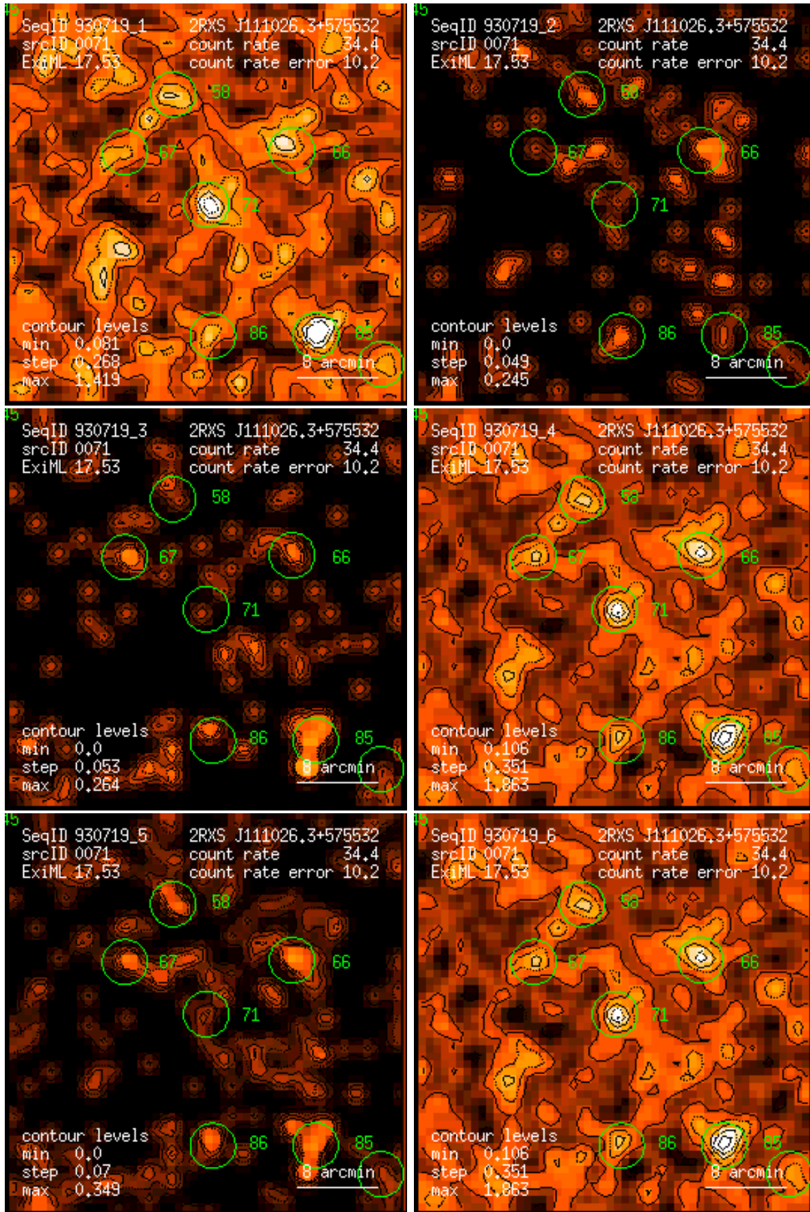
Figure 71: RASS 930719: detection 0071: band rate images, Gaussian filter: (1) PSPC channels 11 – 41, (2) 52 – 90, (3) 91 – 201, (4) 11 – 235, (5) 52 – 201, (6) 11 – 201. Broad band rates in counts/ks. Band rate contour levels in counts/ks/arcmin 2 .
