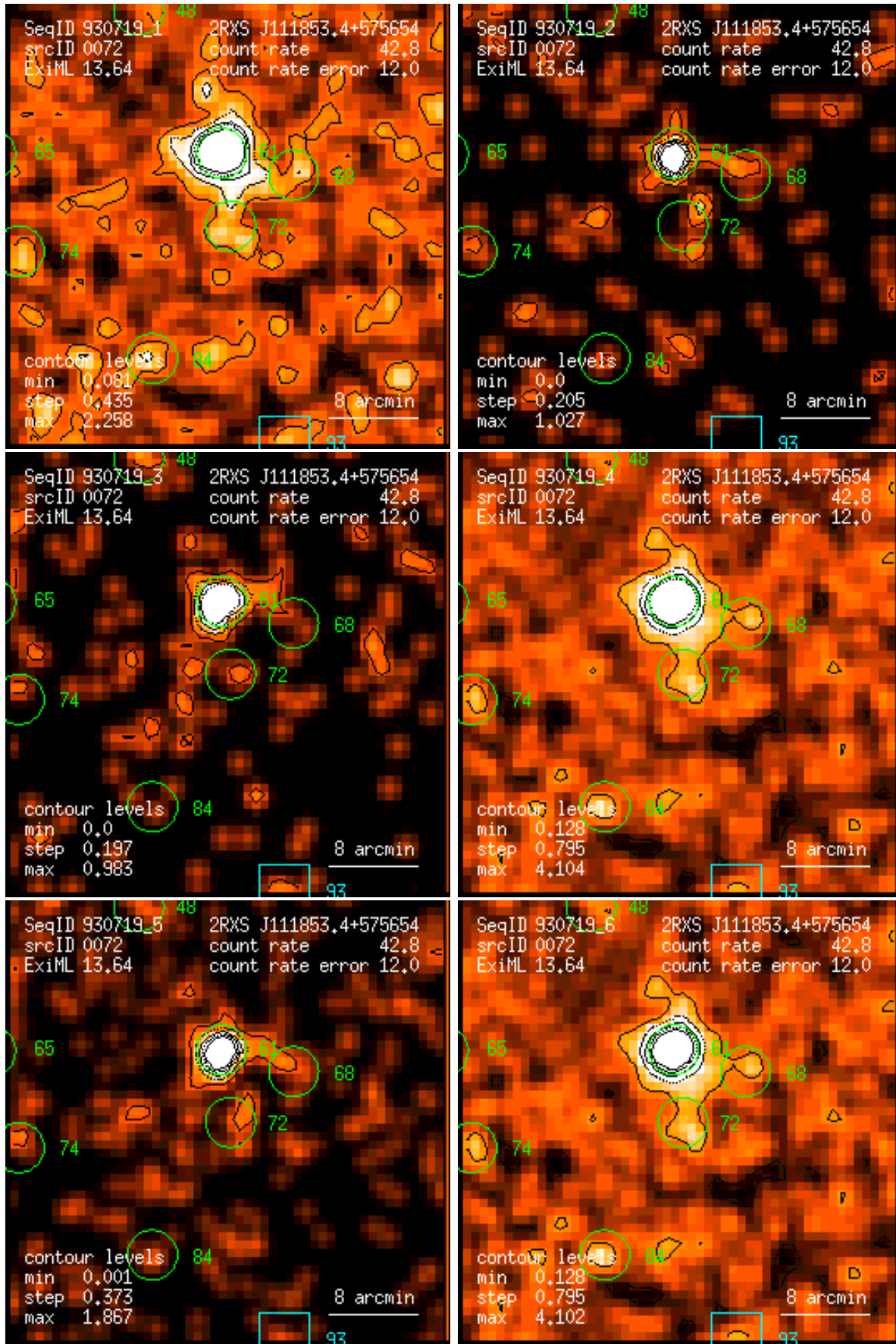
Figure 72: RASS 930719: detection 0072: band rate images, Gaussian filter: (1) PSPC channels 11 – 41, (2) 52 – 90, (3) 91 – 201, (4) 11 – 235, (5) 52 – 201, (6) 11 – 201. Broad band rates in counts/ks. Band rate contour levels in counts/ks/arcmin 2 .
