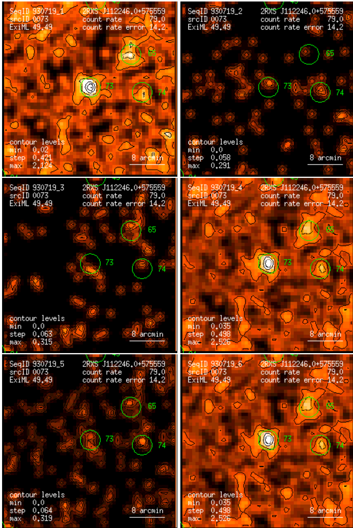
Figure 73: RASS 930719: detection 0073: band rate images, Gaussian filter: (1) PSPC channels 11 – 41, (2) 52 – 90, (3) 91 – 201, (4) 11 – 235, (5) 52 – 201, (6) 11 – 201. Broad band rates in counts/ks. Band rate contour levels in counts/ks/arcmin 2 .
