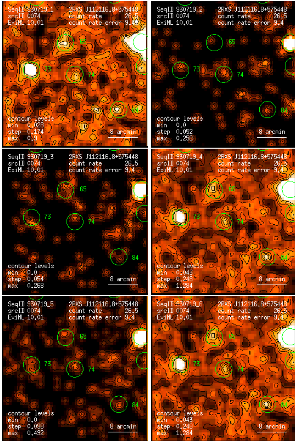
Figure 74: RASS 930719: detection 0074: band rate images, Gaussian filter: (1) PSPC channels 11 – 41, (2) 52 – 90, (3) 91 – 201, (4) 11 – 235, (5) 52 – 201, (6) 11 – 201. Broad band rates in counts/ks. Band rate contour levels in counts/ks/arcmin 2 .
