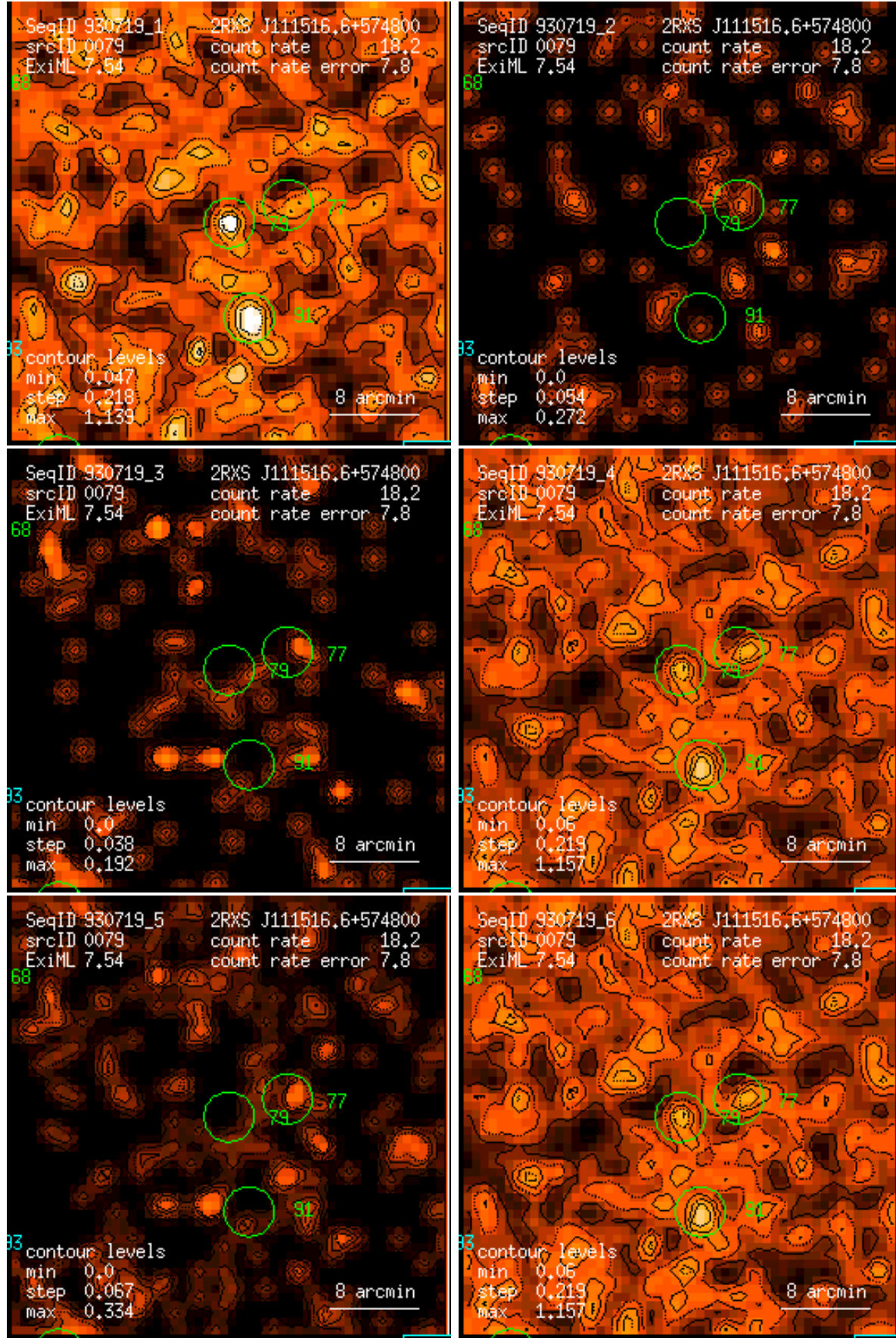
Figure 79: RASS 930719: detection 0079: band rate images, Gaussian filter: (1) PSPC channels 11 – 41, (2) 52 – 90, (3) 91 – 201, (4) 11 – 235, (5) 52 – 201, (6) 11 – 201. Broad band rates in counts/ks. Band rate contour levels in counts/ks/arcmin 2 .
