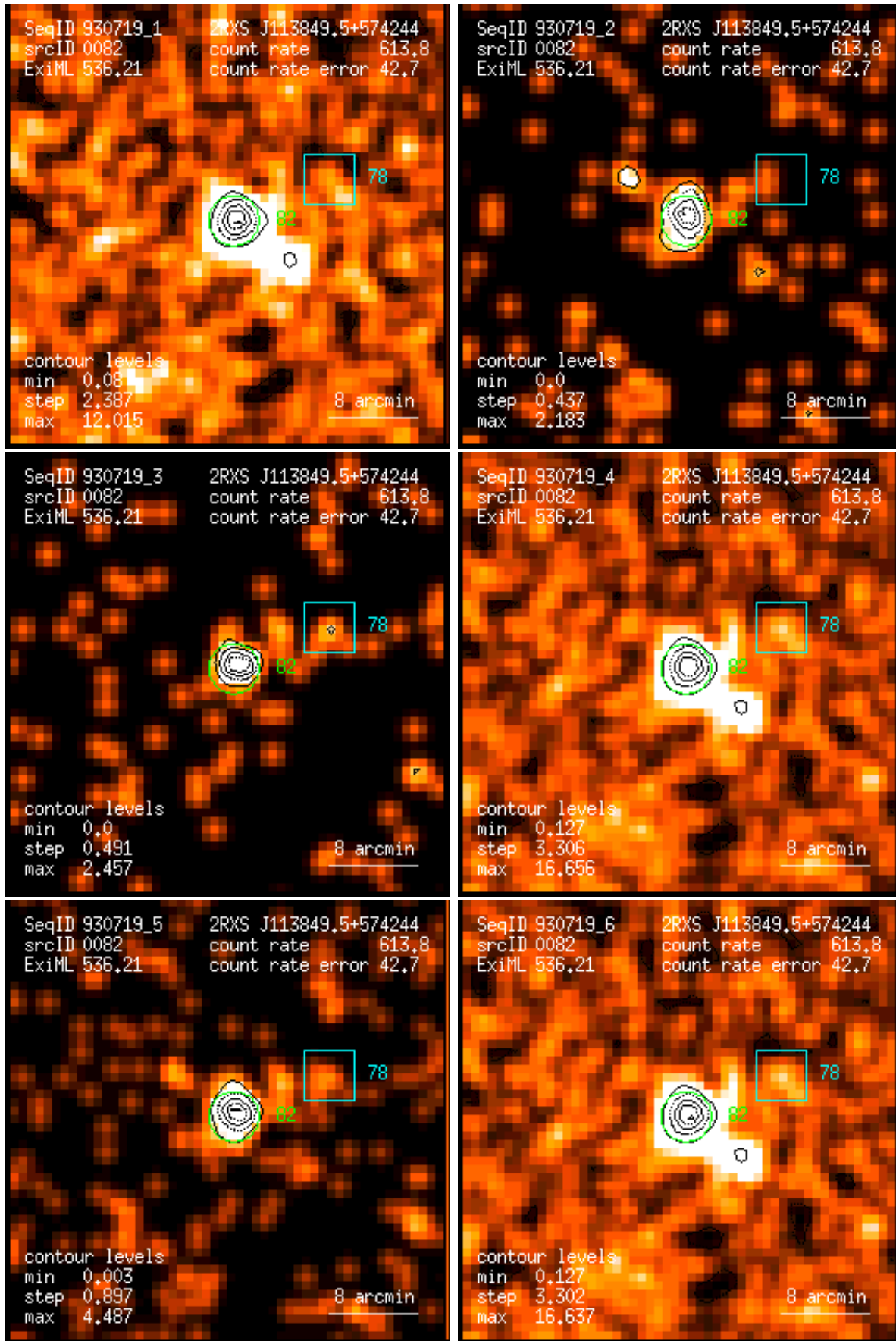
Figure 82: RASS 930719: detection 0082: band rate images, Gaussian filter: (1) PSPC channels 11 – 41, (2) 52 – 90, (3) 91 – 201, (4) 11 – 235, (5) 52 – 201, (6) 11 – 201. Broad band rates in counts/ks. Band rate contour levels in counts/ks/arcmin 2 .
