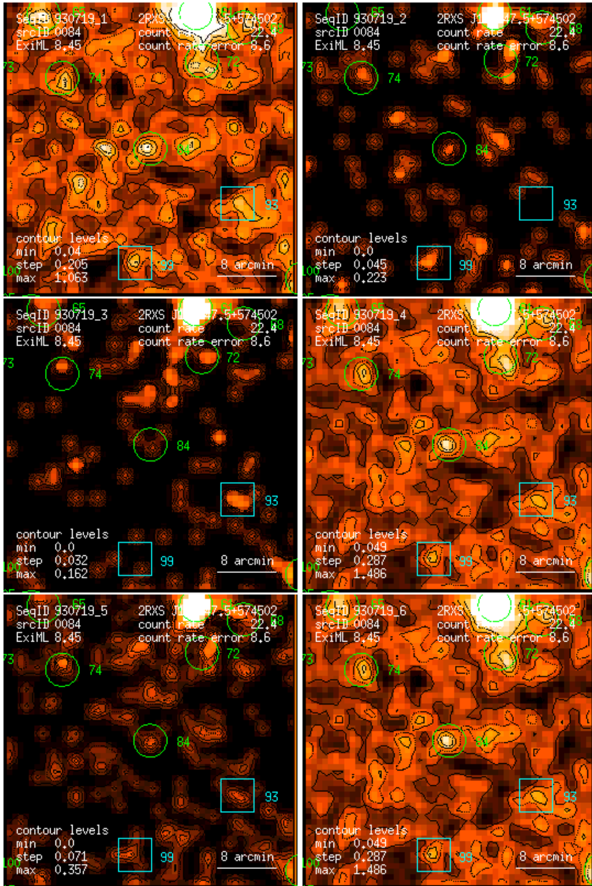
Figure 84: RASS 930719: detection 0084: band rate images, Gaussian filter: (1) PSPC channels 11 – 41, (2) 52 – 90, (3) 91 – 201, (4) 11 – 235, (5) 52 – 201, (6) 11 – 201. Broad band rates in counts/ks. Band rate contour levels in counts/ks/arcmin 2 .
