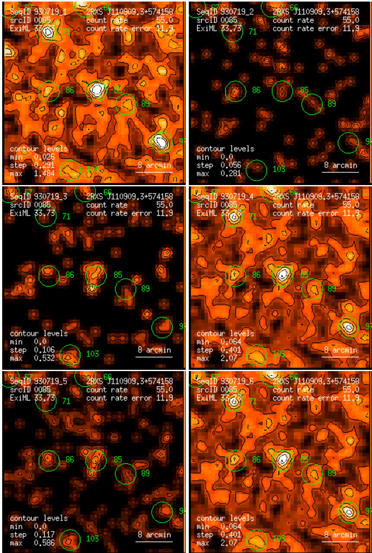
Figure 85: RASS 930719: detection 0085: band rate images, Gaussian filter: (1) PSPC channels 11 – 41, (2) 52 – 90, (3) 91 – 201, (4) 11 – 235, (5) 52 – 201, (6) 11 – 201. Broad band rates in counts/ks. Band rate contour levels in counts/ks/arcmin 2 .
