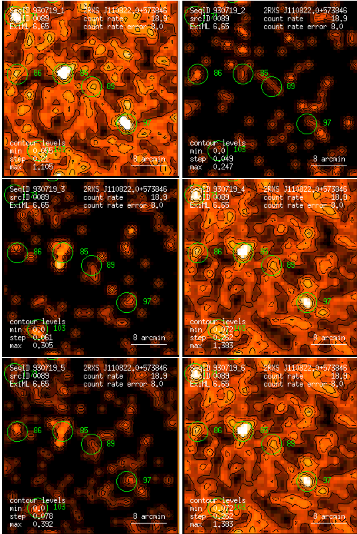
Figure 89: RASS 930719: detection 0089: band rate images, Gaussian filter: (1) PSPC channels 11 – 41, (2) 52 – 90, (3) 91 – 201, (4) 11 – 235, (5) 52 – 201, (6) 11 – 201. Broad band rates in counts/ks. Band rate contour levels in counts/ks/arcmin 2 .
