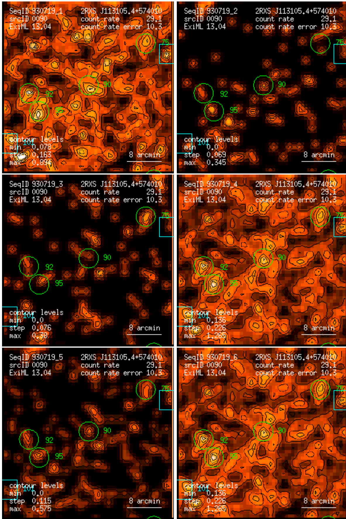
Figure 90: RASS 930719: detection 0090: band rate images, Gaussian filter: (1) PSPC channels 11 – 41, (2) 52 – 90, (3) 91 – 201, (4) 11 – 235, (5) 52 – 201, (6) 11 – 201. Broad band rates in counts/ks. Band rate contour levels in counts/ks/arcmin 2 .
