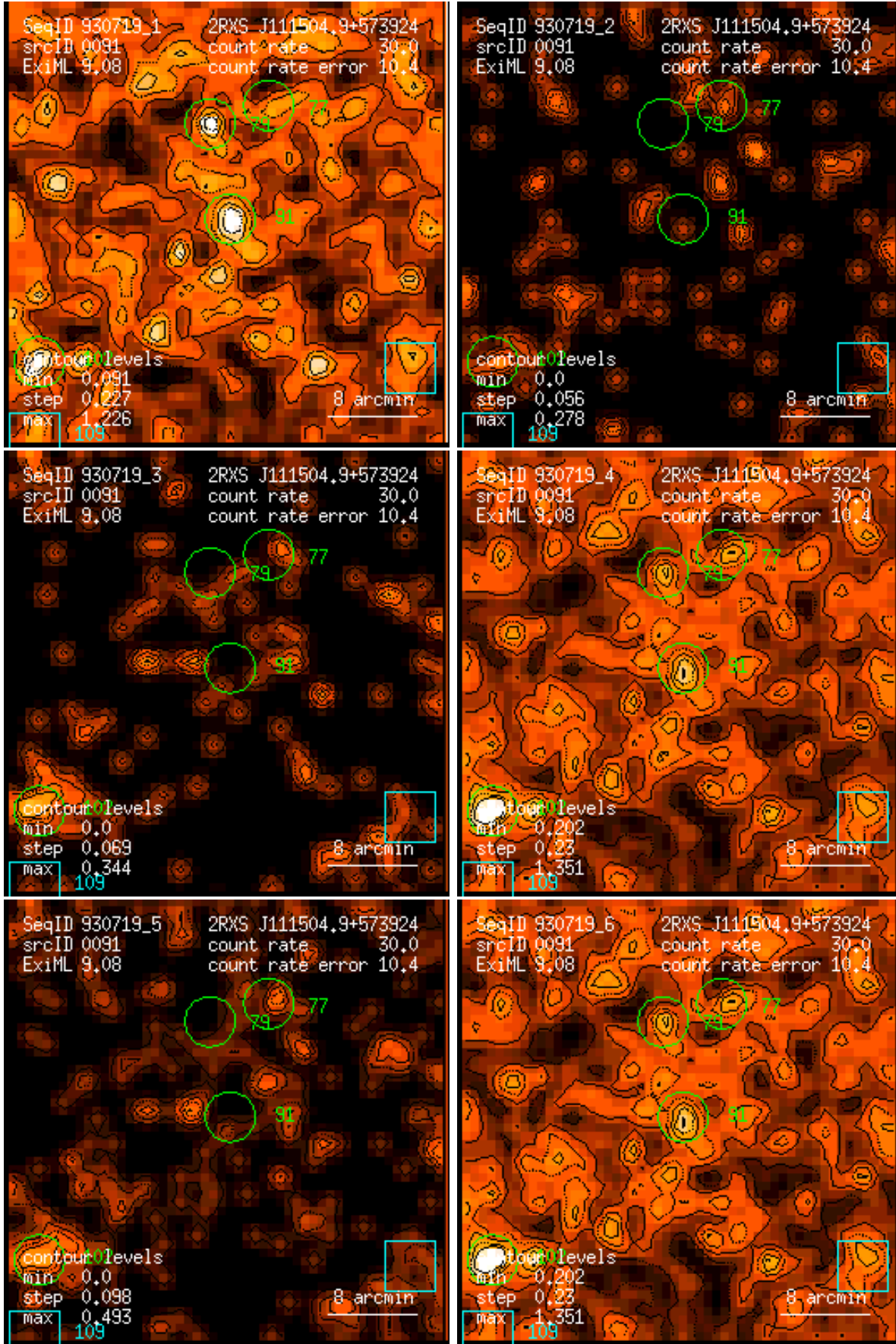
Figure 91: RASS 930719: detection 0091: band rate images, Gaussian filter: (1) PSPC channels 11 – 41, (2) 52 – 90, (3) 91 – 201, (4) 11 – 235, (5) 52 – 201, (6) 11 – 201. Broad band rates in counts/ks. Band rate contour levels in counts/ks/arcmin 2 .
