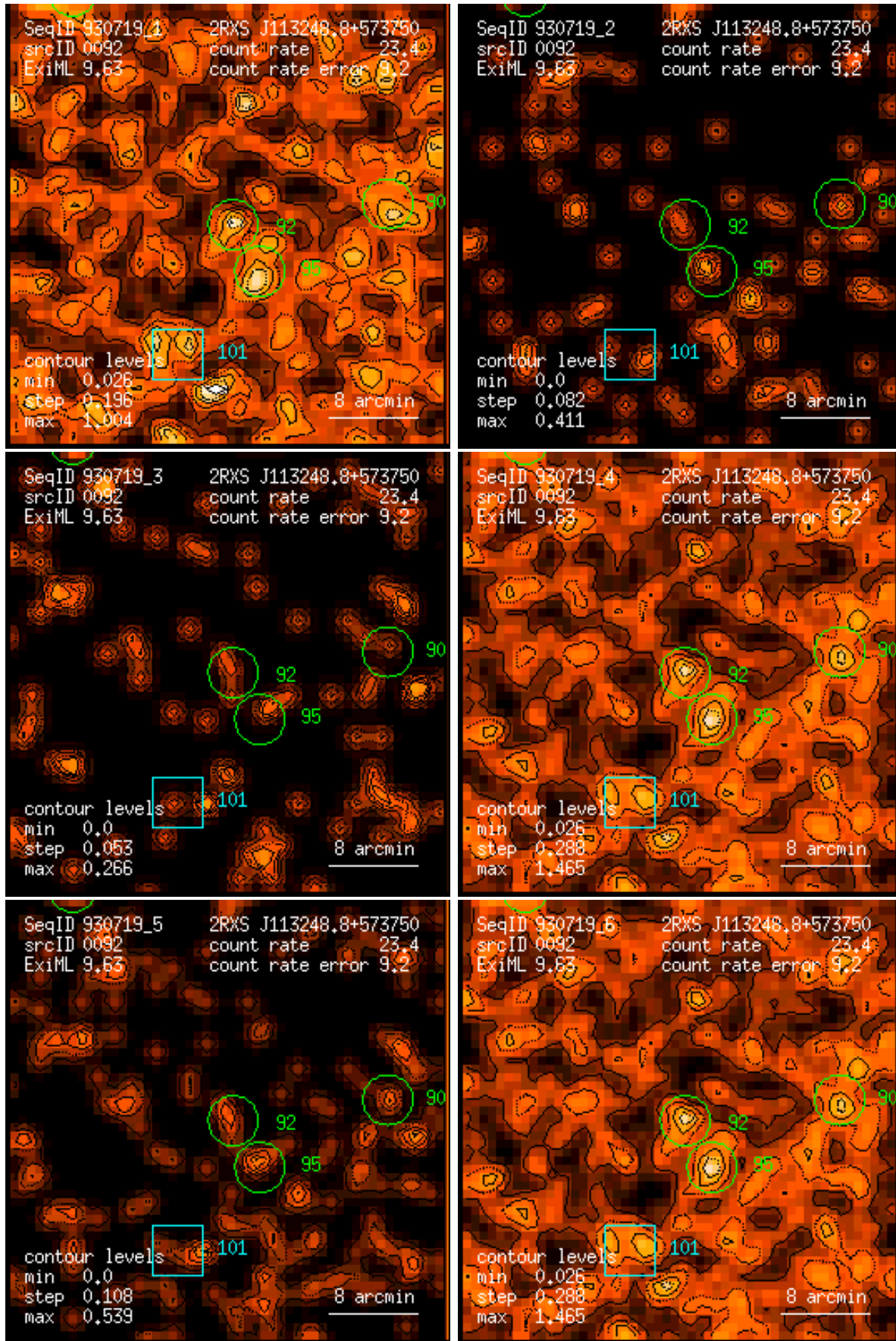
Figure 92: RASS 930719: detection 0092: band rate images, Gaussian filter: (1) PSPC channels 11 – 41, (2) 52 – 90, (3) 91 – 201, (4) 11 – 235, (5) 52 – 201, (6) 11 – 201. Broad band rates in counts/ks. Band rate contour levels in counts/ks/arcmin 2 .
