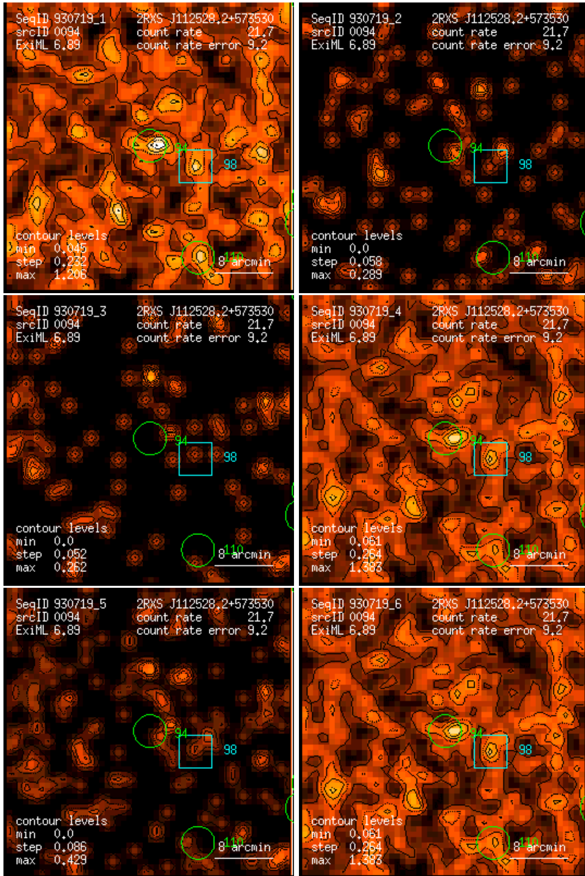
Figure 94: RASS 930719: detection 0094: band rate images, Gaussian filter: (1) PSPC channels 11 – 41, (2) 52 – 90, (3) 91 – 201, (4) 11 – 235, (5) 52 – 201, (6) 11 – 201. Broad band rates in counts/ks. Band rate contour levels in counts/ks/arcmin 2 .
