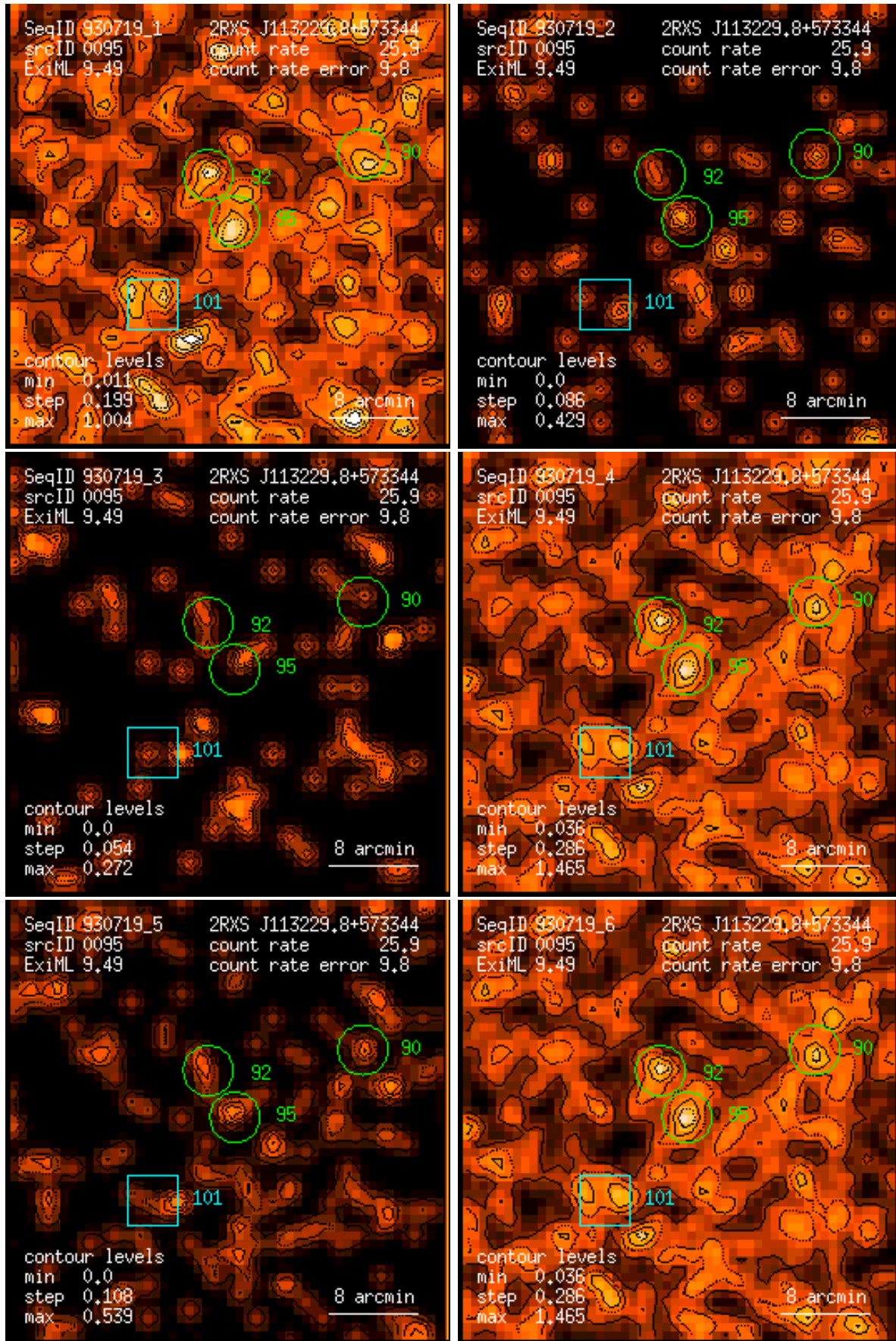
Figure 95: RASS 930719: detection 0095: band rate images, Gaussian filter: (1) PSPC channels 11 – 41, (2) 52 – 90, (3) 91 – 201, (4) 11 – 235, (5) 52 – 201, (6) 11 – 201. Broad band rates in counts/ks. Band rate contour levels in counts/ks/arcmin 2 .
