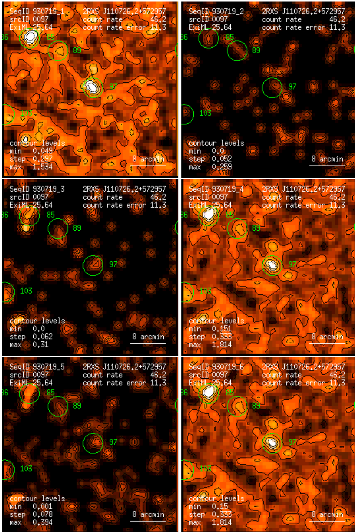
Figure 97: RASS 930719: detection 0097: band rate images, Gaussian filter: (1) PSPC channels 11 – 41, (2) 52 – 90, (3) 91 – 201, (4) 11 – 235, (5) 52 – 201, (6) 11 – 201. Broad band rates in counts/ks. Band rate contour levels in counts/ks/arcmin 2 .
