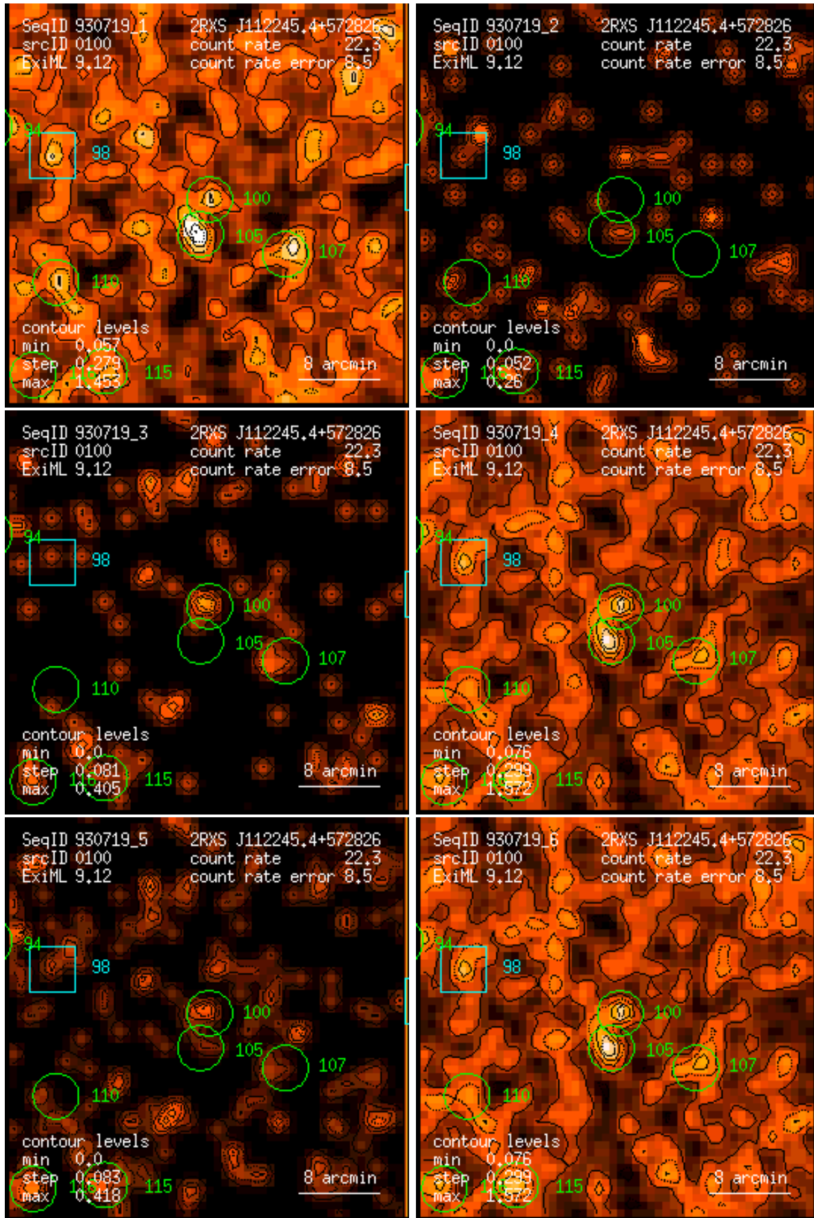
Figure 100: RASS 930719: detection 0100: band rate images, Gaussian filter: (1) PSPC channels 11 – 41, (2) 52 – 90, (3) 91 – 201, (4) 11 – 235, (5) 52 – 201, (6) 11 – 201. Broad band rates in counts/ks. Band rate contour levels in counts/ks/arcmin 2 .
