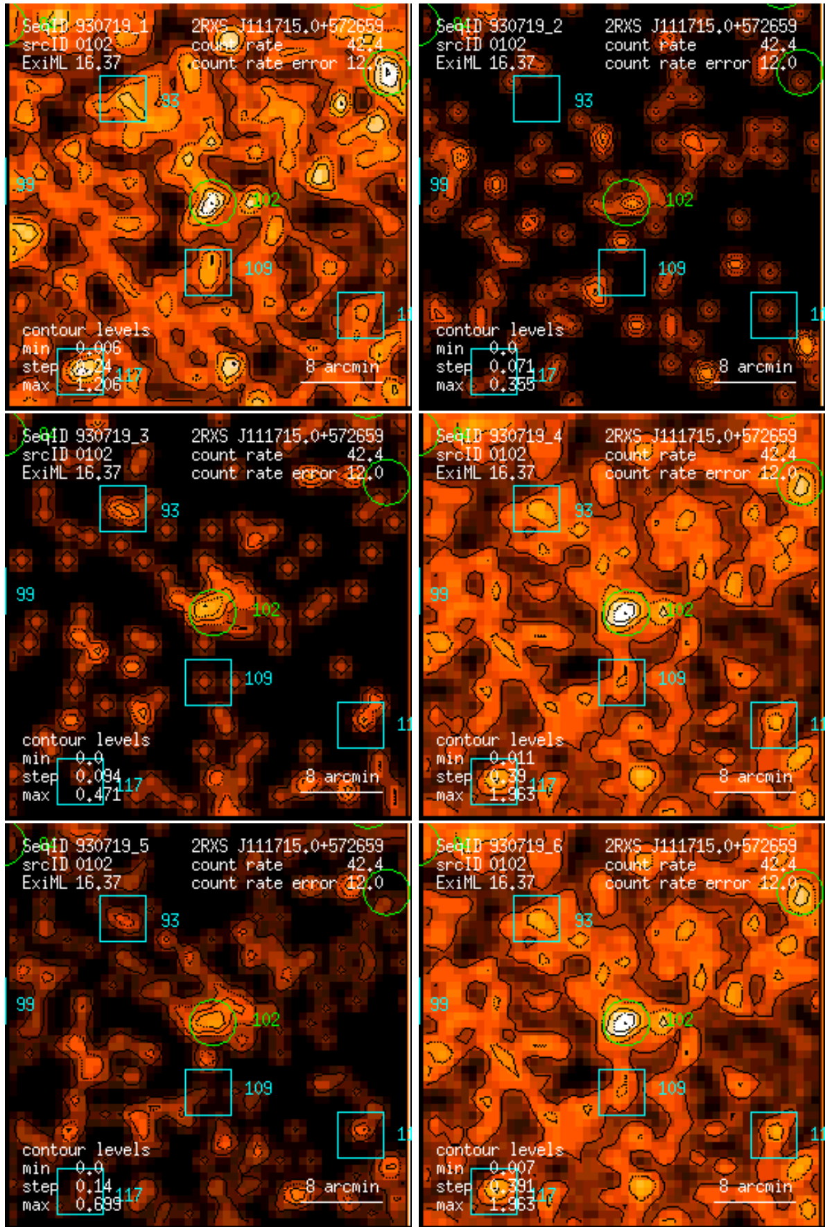
Figure 102: RASS 930719: detection 0102: band rate images, Gaussian filter: (1) PSPC channels 11 – 41, (2) 52 – 90, (3) 91 – 201, (4) 11 – 235, (5) 52 – 201, (6) 11 – 201. Broad band rates in counts/ks. Band rate contour levels in counts/ks/arcmin 2 .
