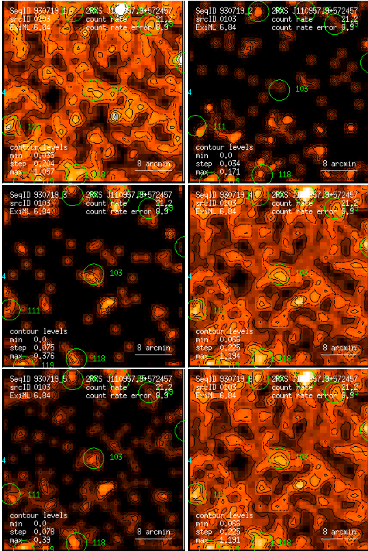
Figure 103: RASS 930719: detection 0103: band rate images, Gaussian filter: (1) PSPC channels 11 – 41, (2) 52 – 90, (3) 91 – 201, (4) 11 – 235, (5) 52 – 201, (6) 11 – 201. Broad band rates in counts/ks. Band rate contour levels in counts/ks/arcmin 2 .
