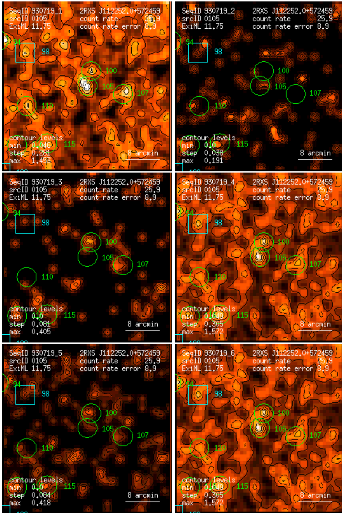
Figure 105: RASS 930719: detection 0105: band rate images, Gaussian filter: (1) PSPC channels 11 – 41, (2) 52 – 90, (3) 91 – 201, (4) 11 – 235, (5) 52 – 201, (6) 11 – 201. Broad band rates in counts/ks. Band rate contour levels in counts/ks/arcmin 2 .
