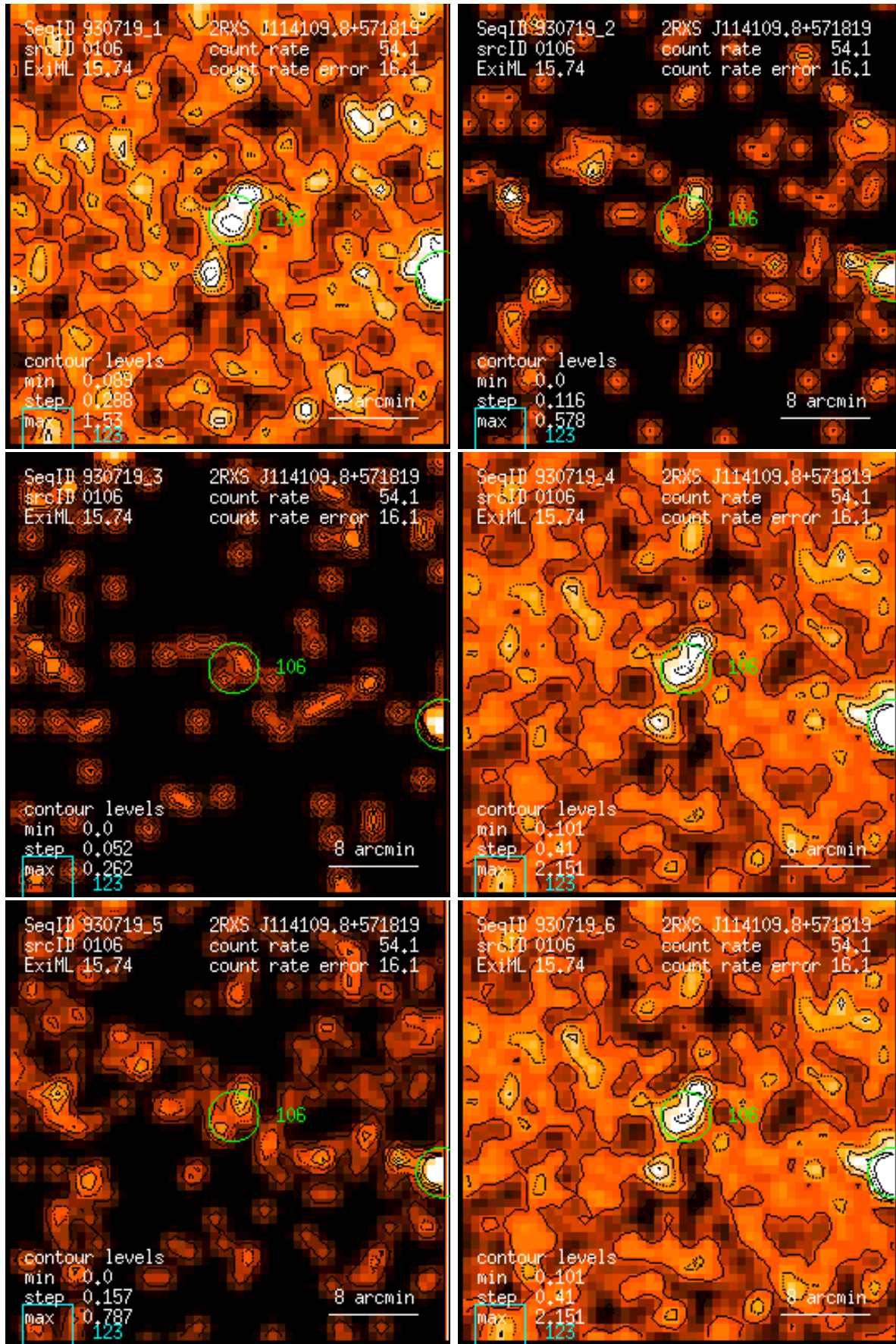
Figure 106: RASS 930719: detection 0106: band rate images, Gaussian filter: (1) PSPC channels 11 – 41, (2) 52 – 90, (3) 91 – 201, (4) 11 – 235, (5) 52 – 201, (6) 11 – 201. Broad band rates in counts/ks. Band rate contour levels in counts/ks/arcmin 2 .
