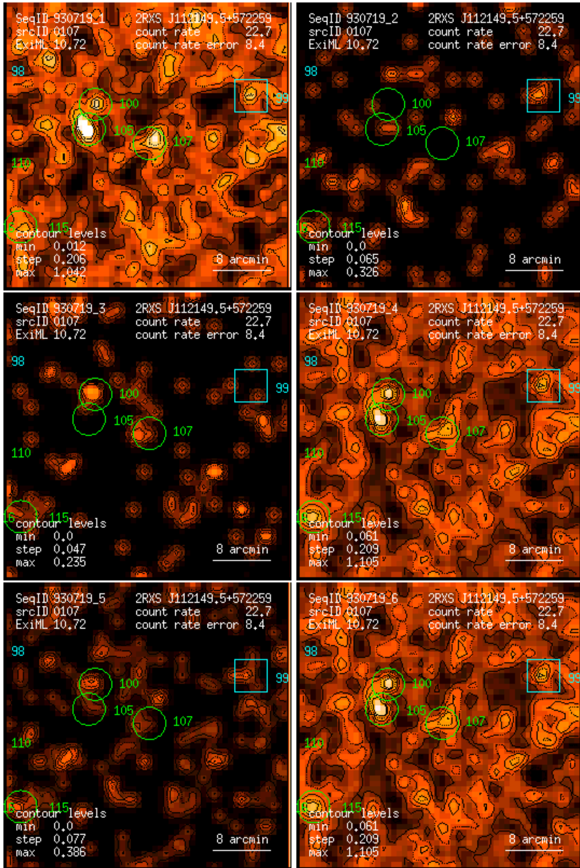
Figure 107: RASS 930719: detection 0107: band rate images, Gaussian filter: (1) PSPC channels 11 – 41, (2) 52 – 90, (3) 91 – 201, (4) 11 – 235, (5) 52 – 201, (6) 11 – 201. Broad band rates in counts/ks. Band rate contour levels in counts/ks/arcmin 2 .
