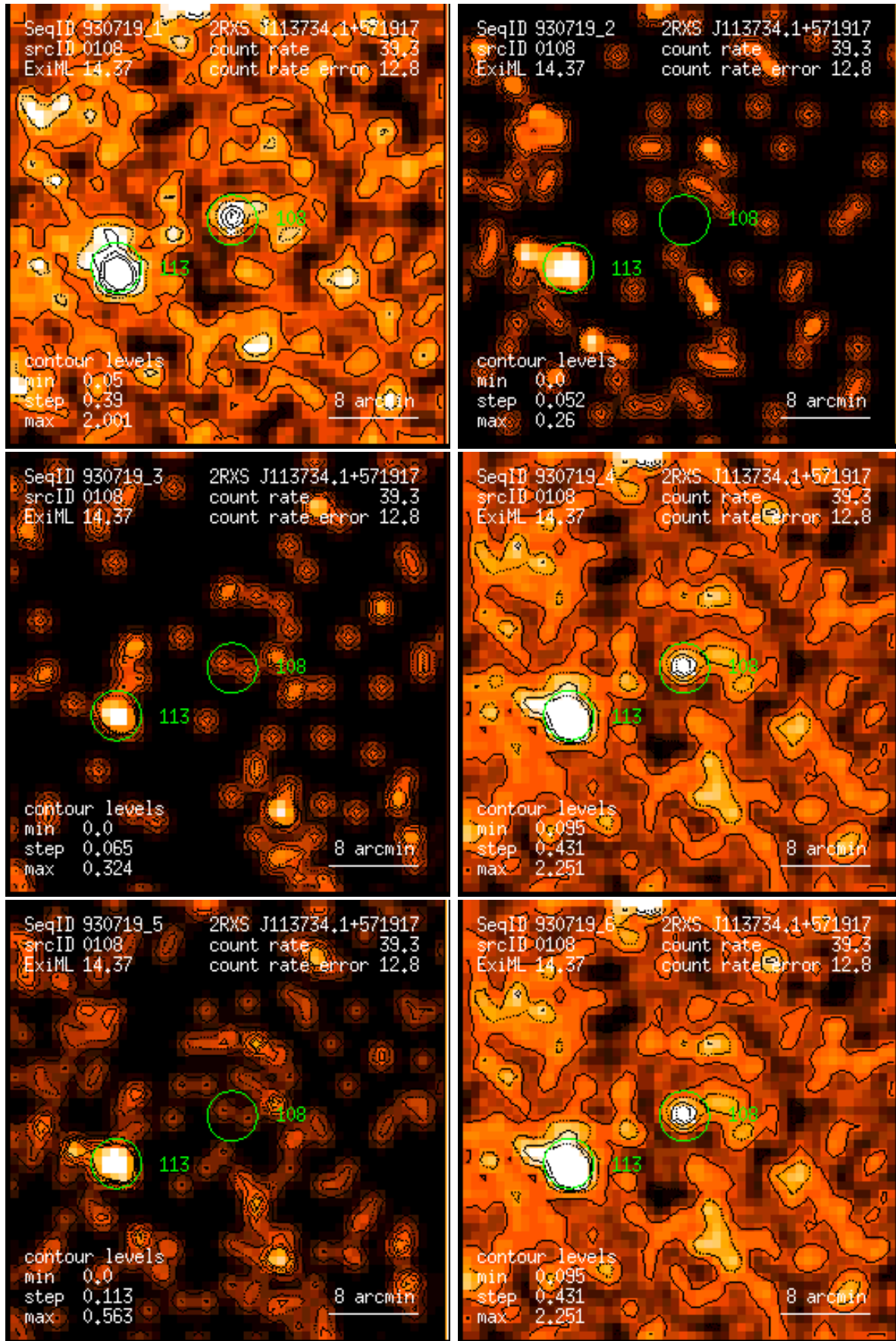
Figure 108: RASS 930719: detection 0108: band rate images, Gaussian filter: (1) PSPC channels 11 – 41, (2) 52 – 90, (3) 91 – 201, (4) 11 – 235, (5) 52 – 201, (6) 11 – 201. Broad band rates in counts/ks. Band rate contour levels in counts/ks/arcmin 2 .
