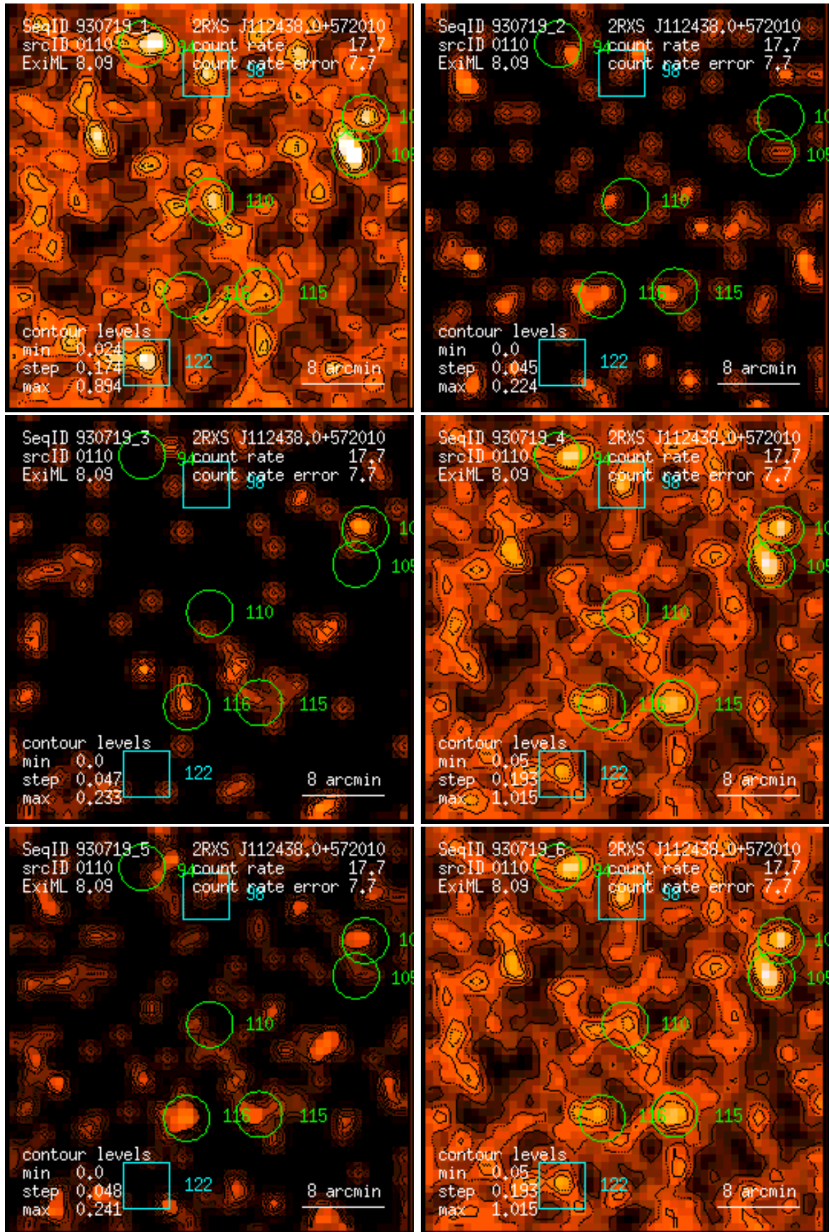
Figure 110: RASS 930719: detection 0110: band rate images, Gaussian filter: (1) PSPC channels 11 – 41, (2) 52 – 90, (3) 91 – 201, (4) 11 – 235, (5) 52 – 201, (6) 11 – 201. Broad band rates in counts/ks. Band rate contour levels in counts/ks/arcmin 2 .
