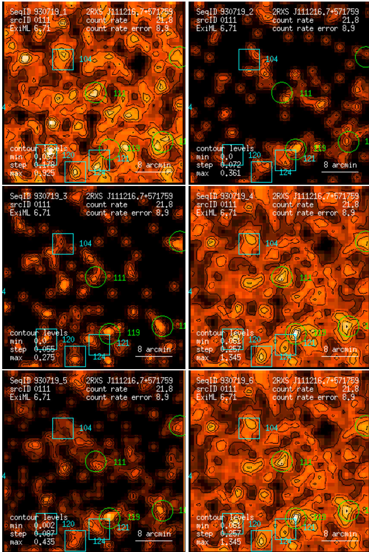
Figure 111: RASS 930719: detection 0111: band rate images, Gaussian filter: (1) PSPC channels 11 – 41, (2) 52 – 90, (3) 91 – 201, (4) 11 – 235, (5) 52 – 201, (6) 11 – 201. Broad band rates in counts/ks. Band rate contour levels in counts/ks/arcmin 2 .
