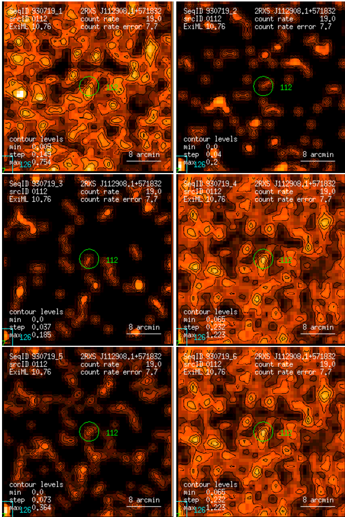
Figure 112: RASS 930719: detection 0112: band rate images, Gaussian filter: (1) PSPC channels 11 – 41, (2) 52 – 90, (3) 91 – 201, (4) 11 – 235, (5) 52 – 201, (6) 11 – 201. Broad band rates in counts/ks. Band rate contour levels in counts/ks/arcmin 2 .
